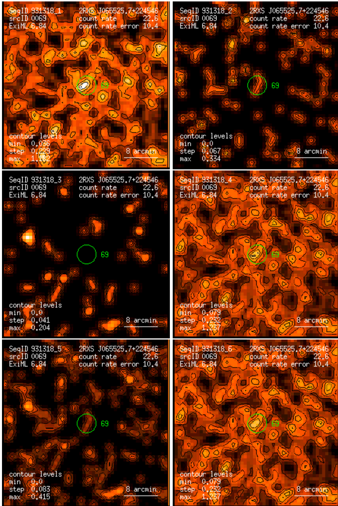
Figure 69: RASS 931318: detection 0069: band rate images, Gaussian filter: (1) PSPC channels 11 – 41, (2) 52 – 90, (3) 91 – 201, (4) 11 – 235, (5) 52 – 201, (6) 11 – 201. Broad band rates in counts/ks. Band rate contour levels in counts/ks/arcmin 2 .
