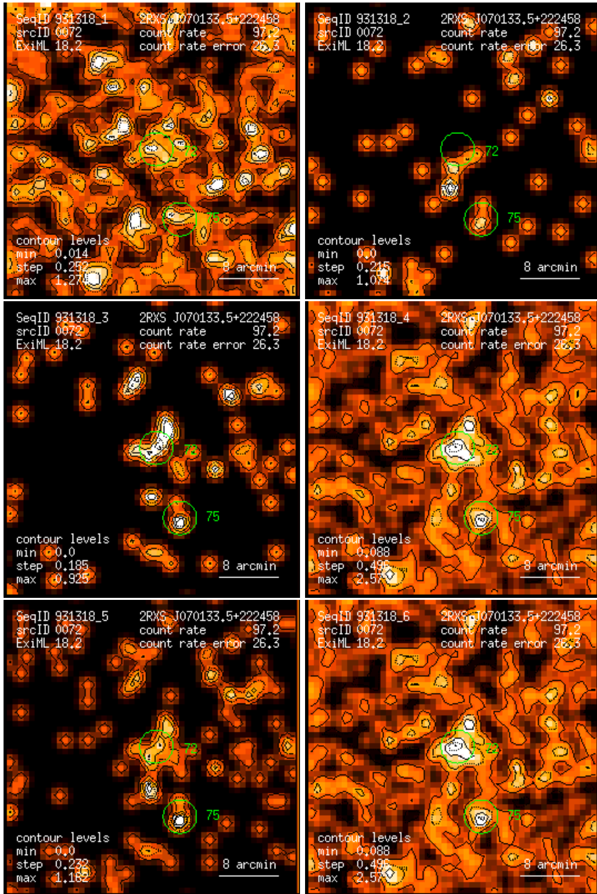
Figure 72: RASS 931318: detection 0072: band rate images, Gaussian filter: (1) PSPC channels 11 – 41, (2) 52 – 90, (3) 91 – 201, (4) 11 – 235, (5) 52 – 201, (6) 11 – 201. Broad band rates in counts/ks. Band rate contour levels in counts/ks/arcmin 2 .
