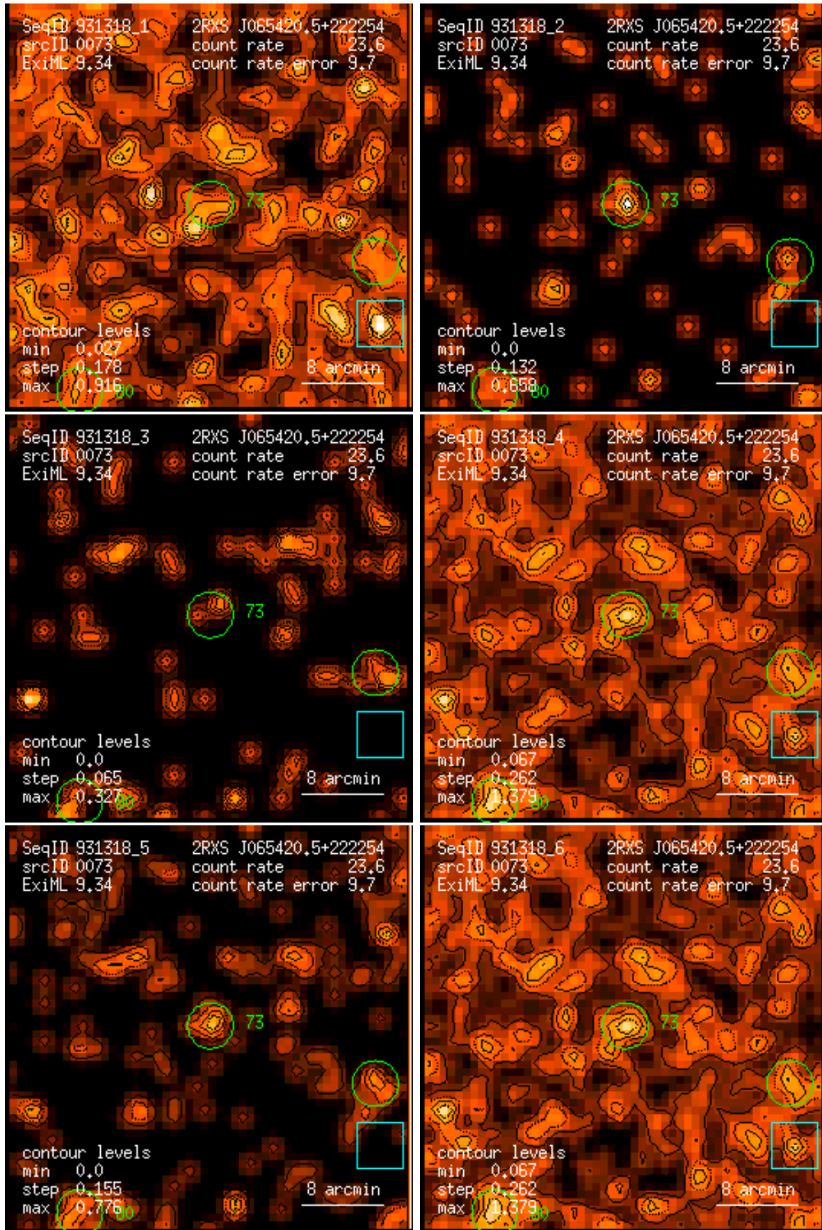
Figure 73: RASS 931318: detection 0073: band rate images, Gaussian filter: (1) PSPC channels 11 – 41, (2) 52 – 90, (3) 91 – 201, (4) 11 – 235, (5) 52 – 201, (6) 11 – 201. Broad band rates in counts/ks. Band rate contour levels in counts/ks/arcmin 2 .
