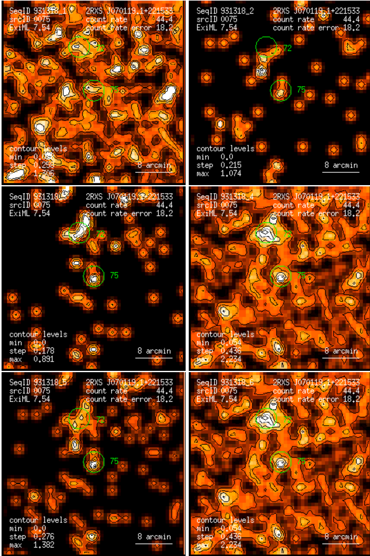
Figure 75: RASS 931318: detection 0075: band rate images, Gaussian filter: (1) PSPC channels 11 – 41, (2) 52 – 90, (3) 91 – 201, (4) 11 – 235, (5) 52 – 201, (6) 11 – 201. Broad band rates in counts/ks. Band rate contour levels in counts/ks/arcmin 2 .
