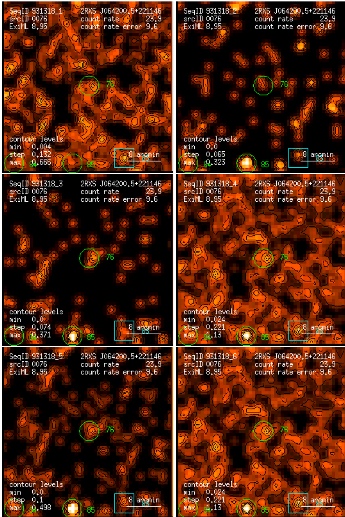
Figure 76: RASS 931318: detection 0076: band rate images, Gaussian filter: (1) PSPC channels 11 – 41, (2) 52 – 90, (3) 91 – 201, (4) 11 – 235, (5) 52 – 201, (6) 11 – 201. Broad band rates in counts/ks. Band rate contour levels in counts/ks/arcmin 2 .
