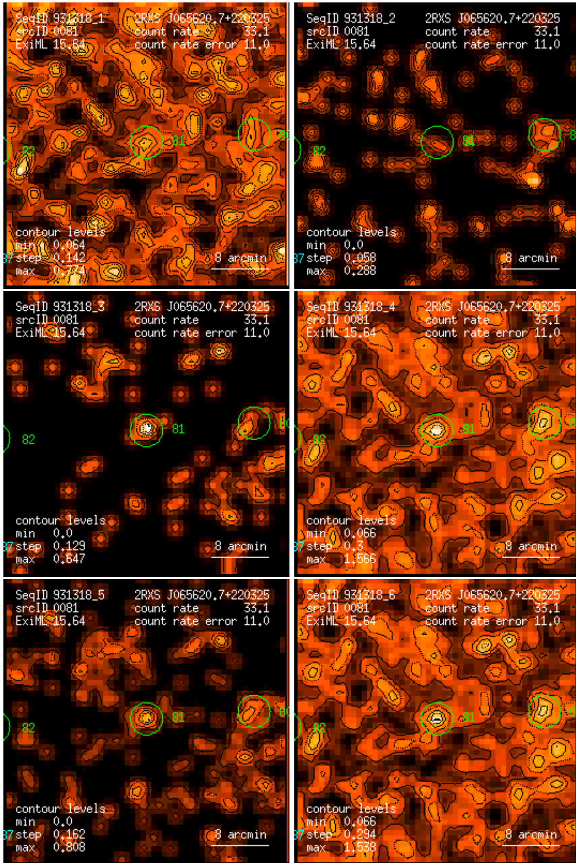
Figure 81: RASS 931318: detection 0081: band rate images, Gaussian filter: (1) PSPC channels 11 – 41, (2) 52 – 90, (3) 91 – 201, (4) 11 – 235, (5) 52 – 201, (6) 11 – 201. Broad band rates in counts/ks. Band rate contour levels in counts/ks/arcmin 2 .
