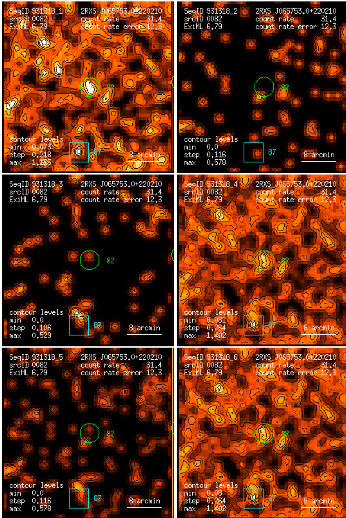
Figure 82: RASS 931318: detection 0082: band rate images, Gaussian filter: (1) PSPC channels 11 – 41, (2) 52 – 90, (3) 91 – 201, (4) 11 – 235, (5) 52 – 201, (6) 11 – 201. Broad band rates in counts/ks. Band rate contour levels in counts/ks/arcmin 2 .
