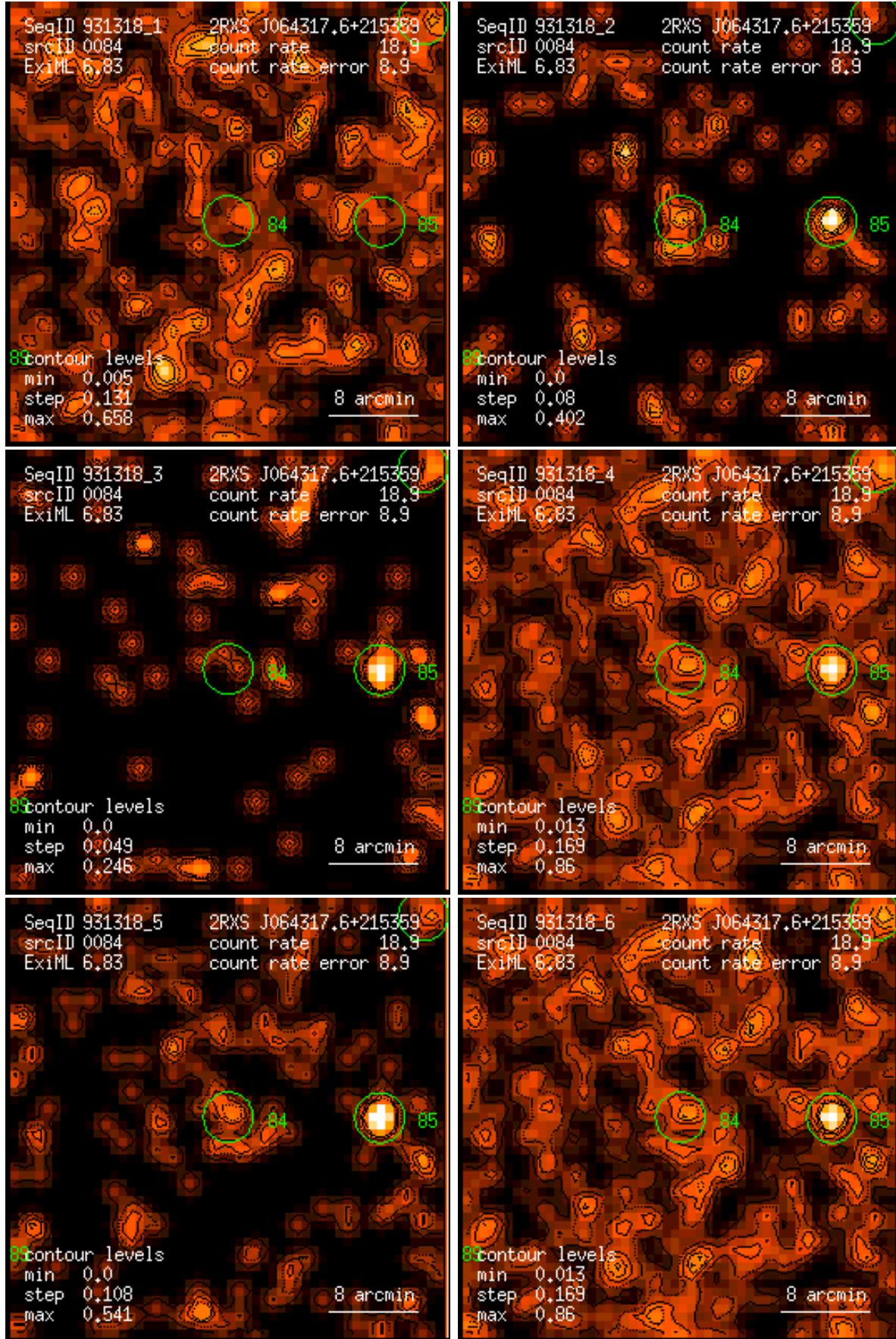
Figure 84: RASS 931318: detection 0084: band rate images, Gaussian filter: (1) PSPC channels 11 – 41, (2) 52 – 90, (3) 91 – 201, (4) 11 – 235, (5) 52 – 201, (6) 11 – 201. Broad band rates in counts/ks. Band rate contour levels in counts/ks/arcmin 2 .
