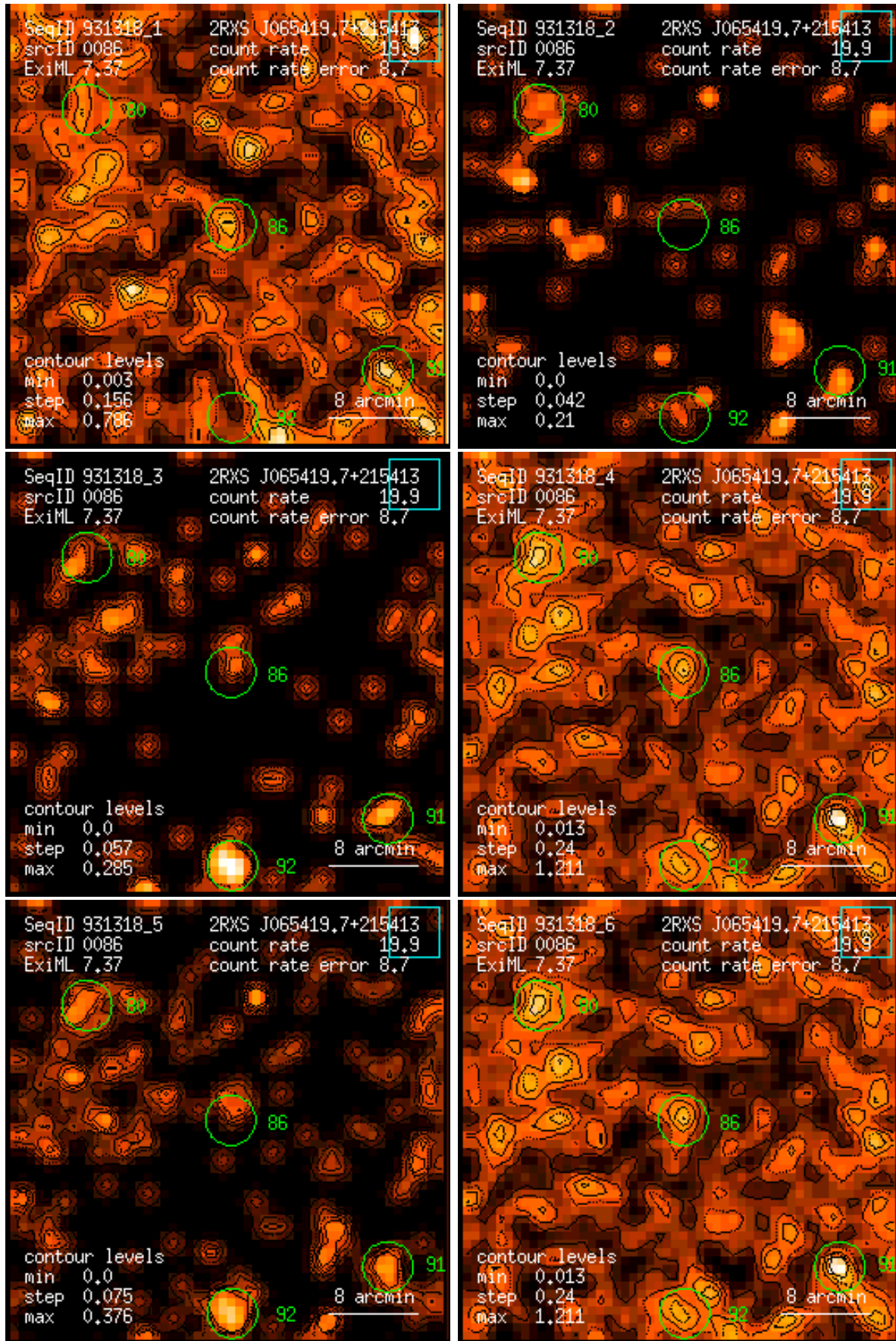
Figure 86: RASS 931318: detection 0086: band rate images, Gaussian filter: (1) PSPC channels 11 – 41, (2) 52 – 90, (3) 91 – 201, (4) 11 – 235, (5) 52 – 201, (6) 11 – 201. Broad band rates in counts/ks. Band rate contour levels in counts/ks/arcmin 2 .
