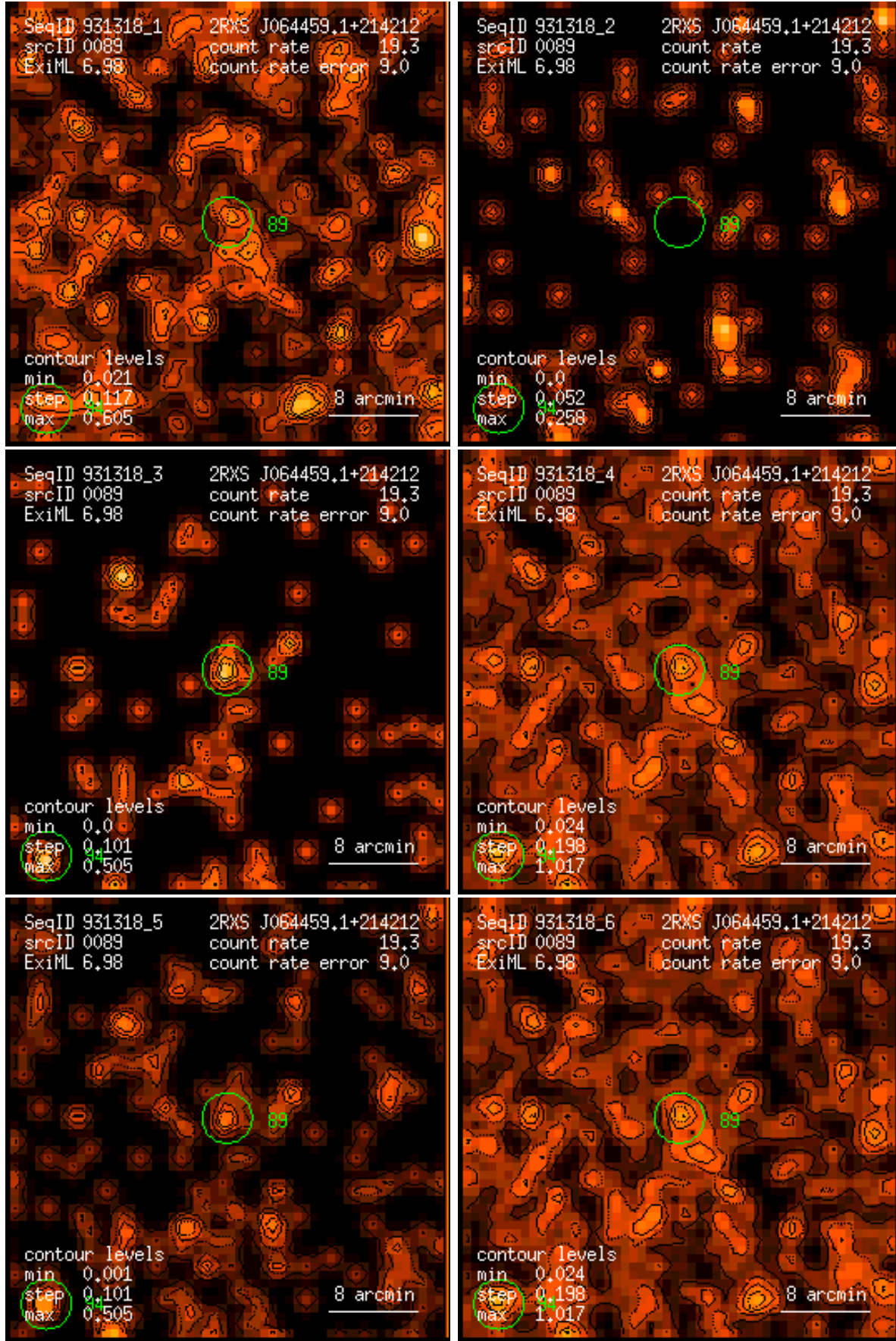
Figure 89: RASS 931318: detection 0089: band rate images, Gaussian filter: (1) PSPC channels 11 – 41, (2) 52 – 90, (3) 91 – 201, (4) 11 – 235, (5) 52 – 201, (6) 11 – 201. Broad band rates in counts/ks. Band rate contour levels in counts/ks/arcmin 2 .
