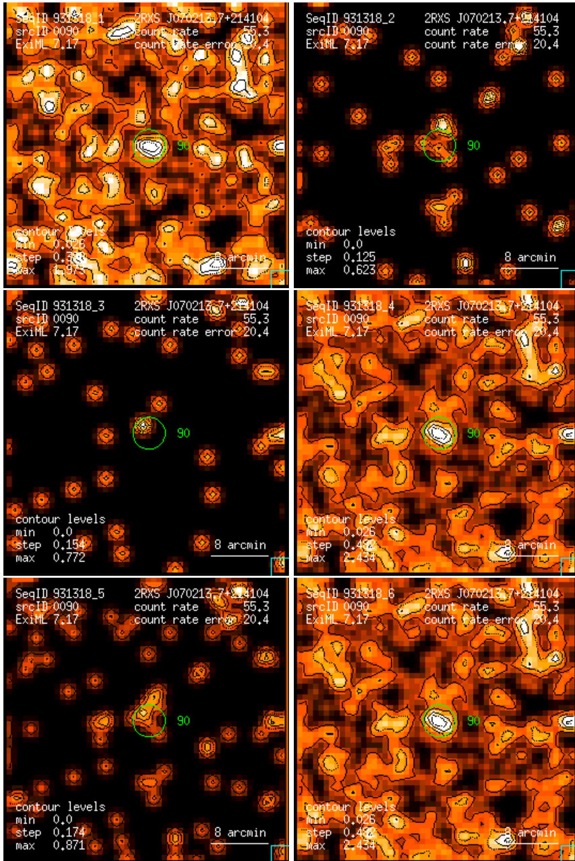
Figure 90: RASS 931318: detection 0090: band rate images, Gaussian filter: (1) PSPC channels 11 – 41, (2) 52 – 90, (3) 91 – 201, (4) 11 – 235, (5) 52 – 201, (6) 11 – 201. Broad band rates in counts/ks. Band rate contour levels in counts/ks/arcmin 2 .
