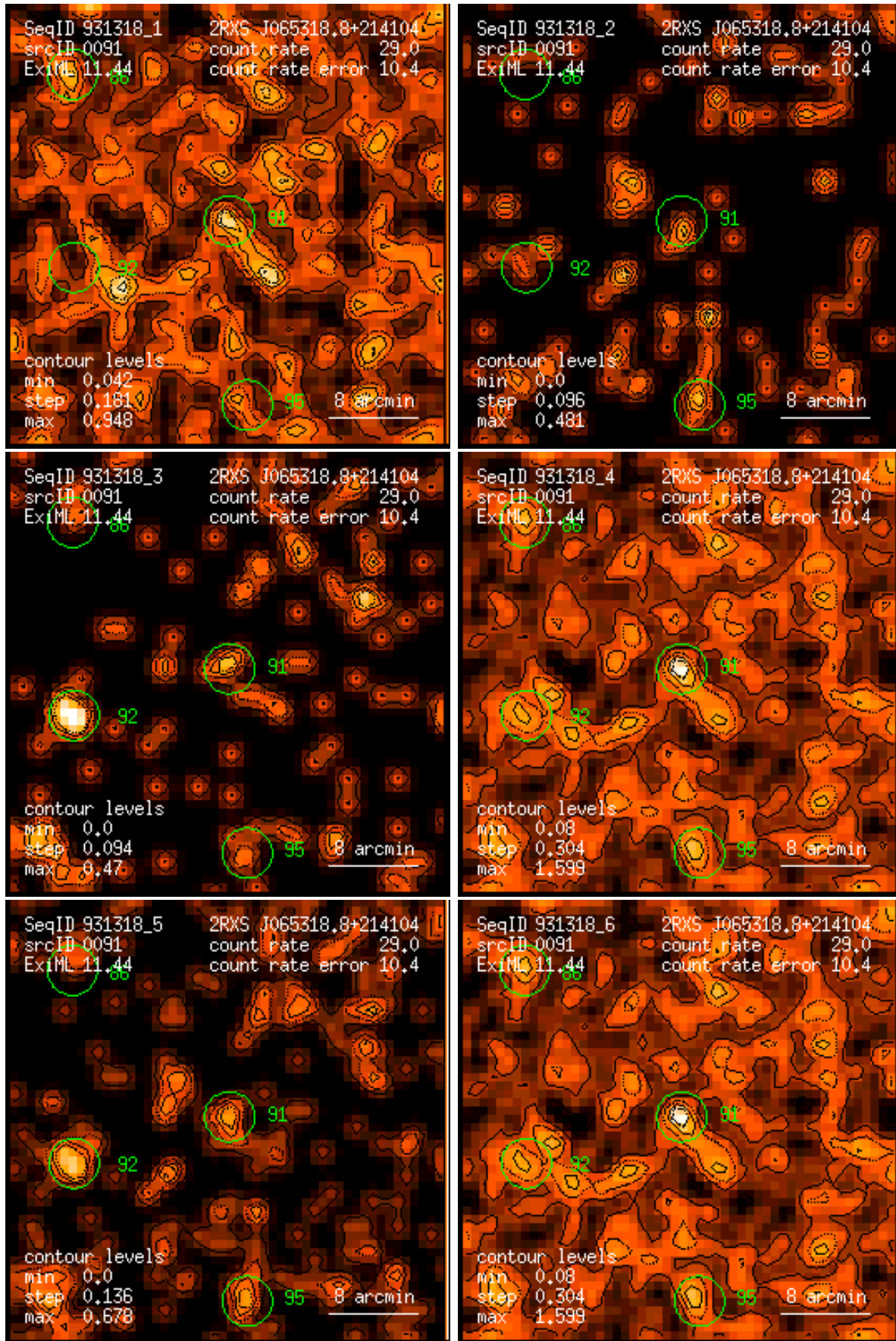
Figure 91: RASS 931318: detection 0091: band rate images, Gaussian filter: (1) PSPC channels 11 – 41, (2) 52 – 90, (3) 91 – 201, (4) 11 – 235, (5) 52 – 201, (6) 11 – 201. Broad band rates in counts/ks. Band rate contour levels in counts/ks/arcmin 2 .
