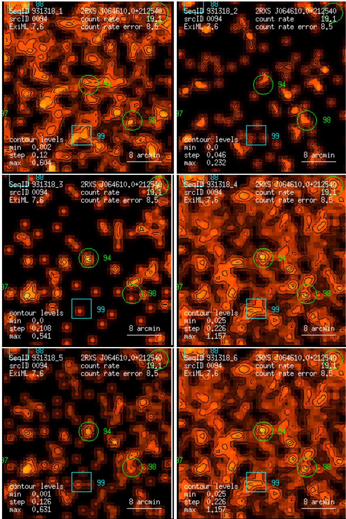
Figure 94: RASS 931318: detection 0094: band rate images, Gaussian filter: (1) PSPC channels 11 – 41, (2) 52 – 90, (3) 91 – 201, (4) 11 – 235, (5) 52 – 201, (6) 11 – 201. Broad band rates in counts/ks. Band rate contour levels in counts/ks/arcmin 2 .
