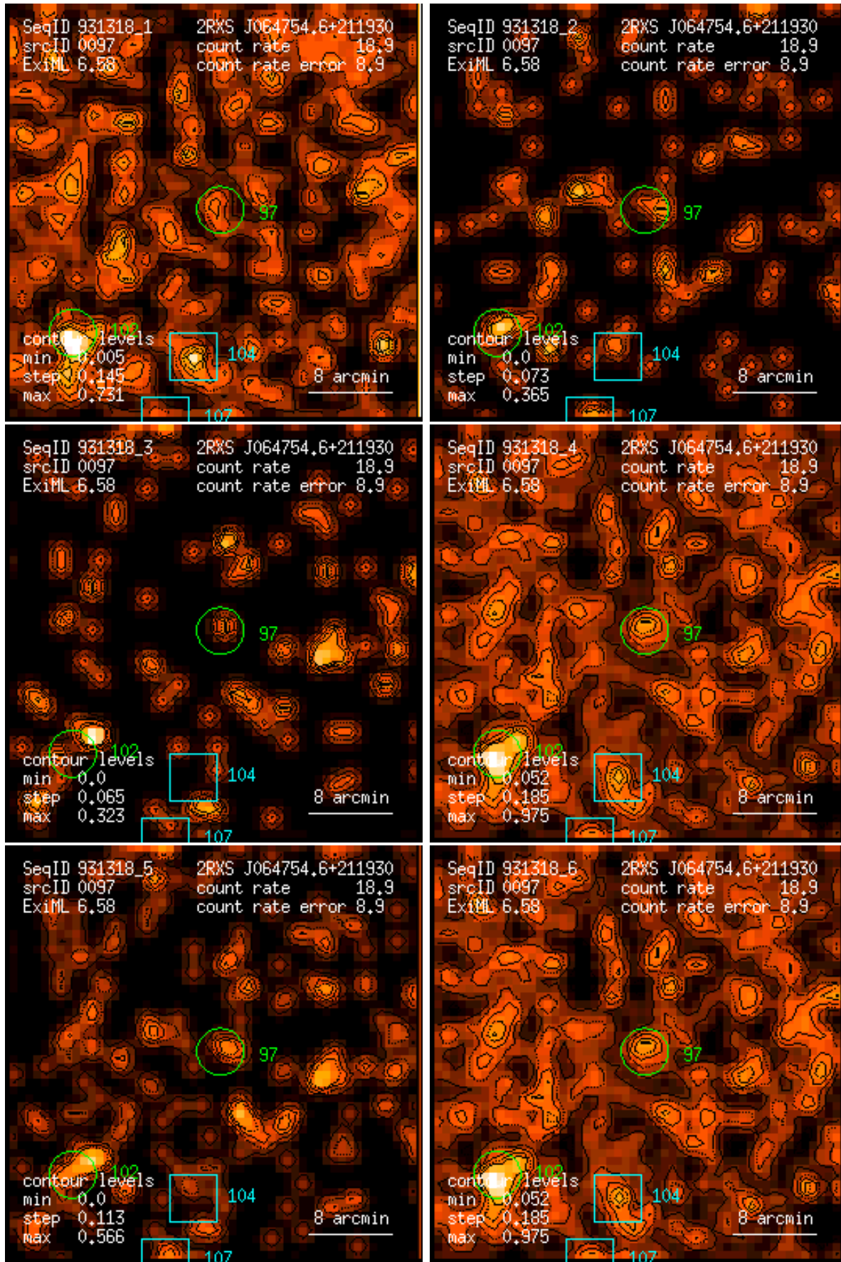
Figure 97: RASS 931318: detection 0097: band rate images, Gaussian filter: (1) PSPC channels 11 – 41, (2) 52 – 90, (3) 91 – 201, (4) 11 – 235, (5) 52 – 201, (6) 11 – 201. Broad band rates in counts/ks. Band rate contour levels in counts/ks/arcmin 2 .
