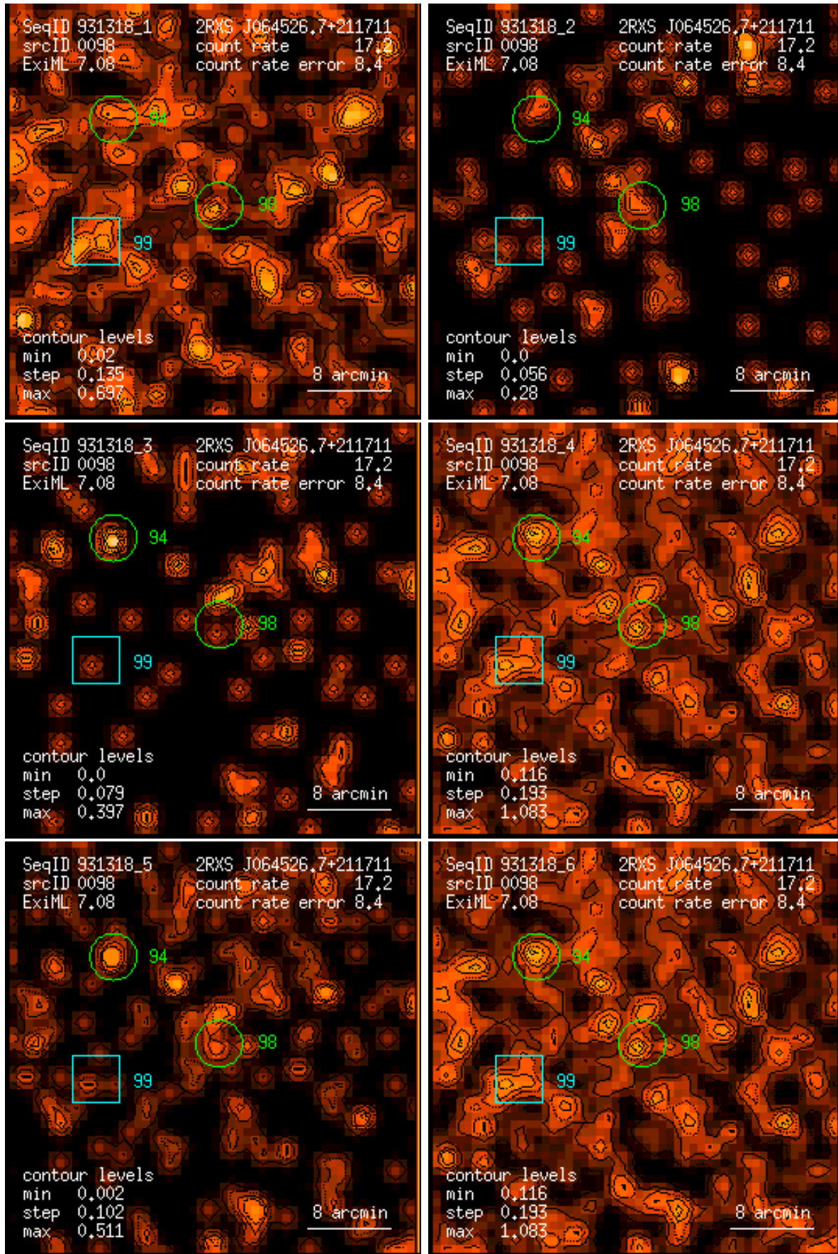
Figure 98: RASS 931318: detection 0098: band rate images, Gaussian filter: (1) PSPC channels 11 – 41, (2) 52 – 90, (3) 91 – 201, (4) 11 – 235, (5) 52 – 201, (6) 11 – 201. Broad band rates in counts/ks. Band rate contour levels in counts/ks/arcmin 2 .
