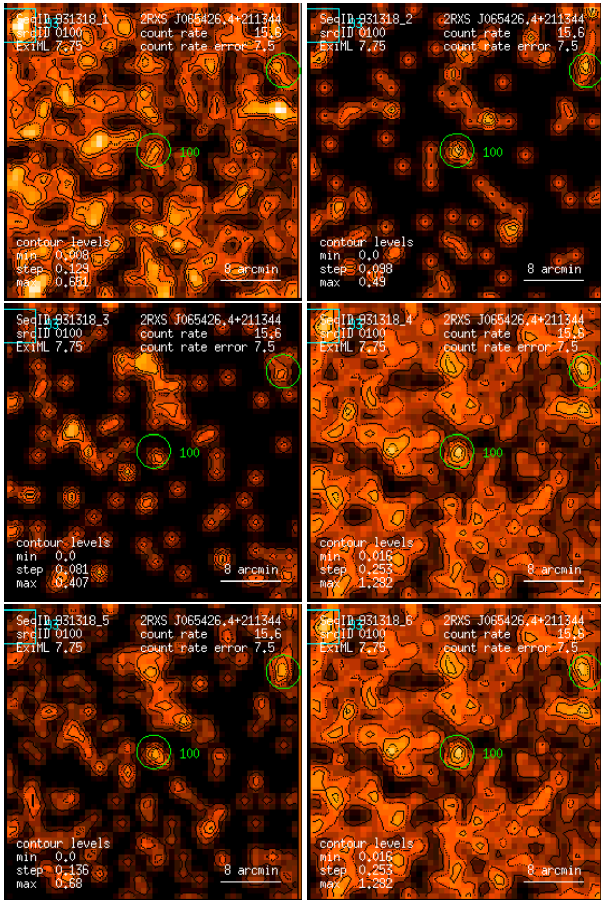
Figure 100: RASS 931318: detection 0100: band rate images, Gaussian filter: (1) PSPC channels 11 – 41, (2) 52 – 90, (3) 91 – 201, (4) 11 – 235, (5) 52 – 201, (6) 11 – 201. Broad band rates in counts/ks. Band rate contour levels in counts/ks/arcmin 2 .
