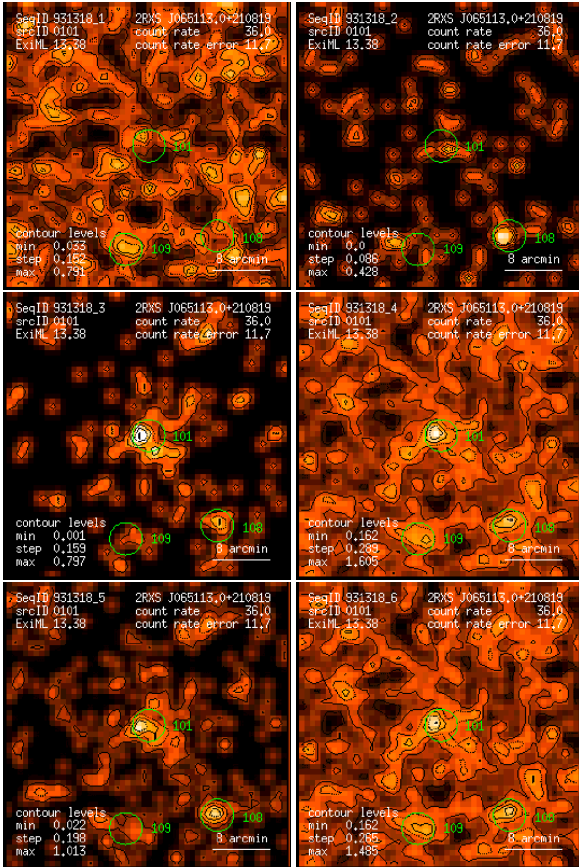
Figure 101: RASS 931318: detection 0101: band rate images, Gaussian filter: (1) PSPC channels 11 – 41, (2) 52 – 90, (3) 91 – 201, (4) 11 – 235, (5) 52 – 201, (6) 11 – 201. Broad band rates in counts/ks. Band rate contour levels in counts/ks/arcmin 2 .
