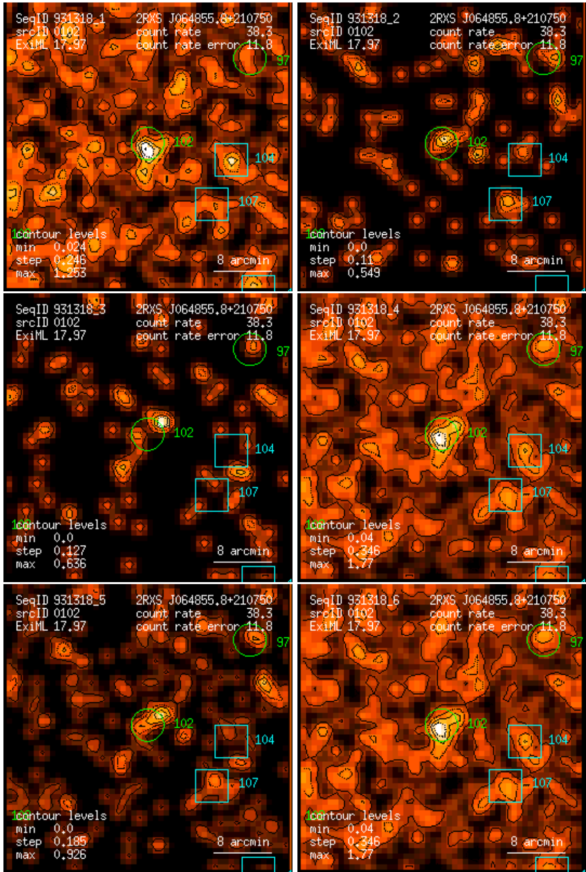
Figure 102: RASS 931318: detection 0102: band rate images, Gaussian filter: (1) PSPC channels 11 – 41, (2) 52 – 90, (3) 91 – 201, (4) 11 – 235, (5) 52 – 201, (6) 11 – 201. Broad band rates in counts/ks. Band rate contour levels in counts/ks/arcmin 2 .
