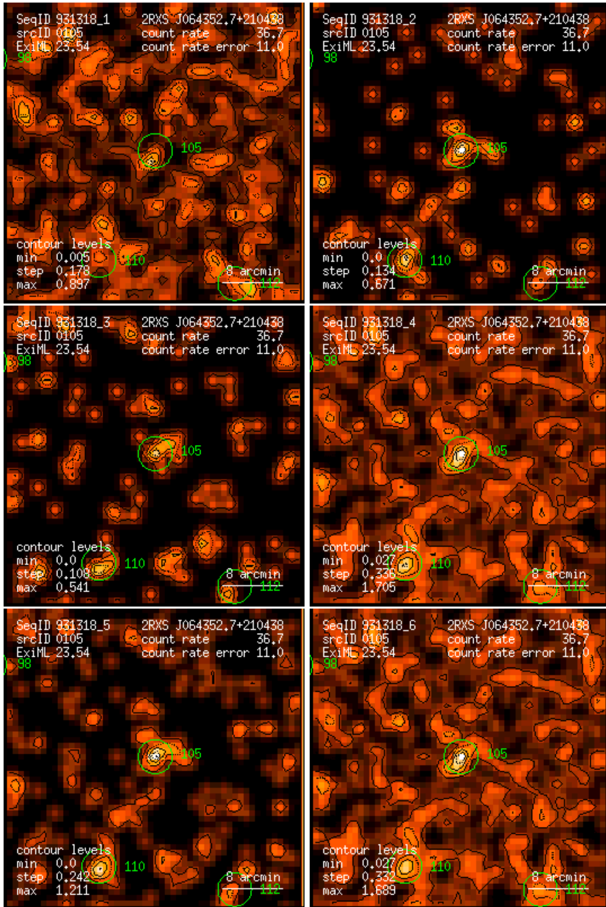
Figure 105: RASS 931318: detection 0105: band rate images, Gaussian filter: (1) PSPC channels 11 – 41, (2) 52 – 90, (3) 91 – 201, (4) 11 – 235, (5) 52 – 201, (6) 11 – 201. Broad band rates in counts/ks. Band rate contour levels in counts/ks/arcmin 2 .
