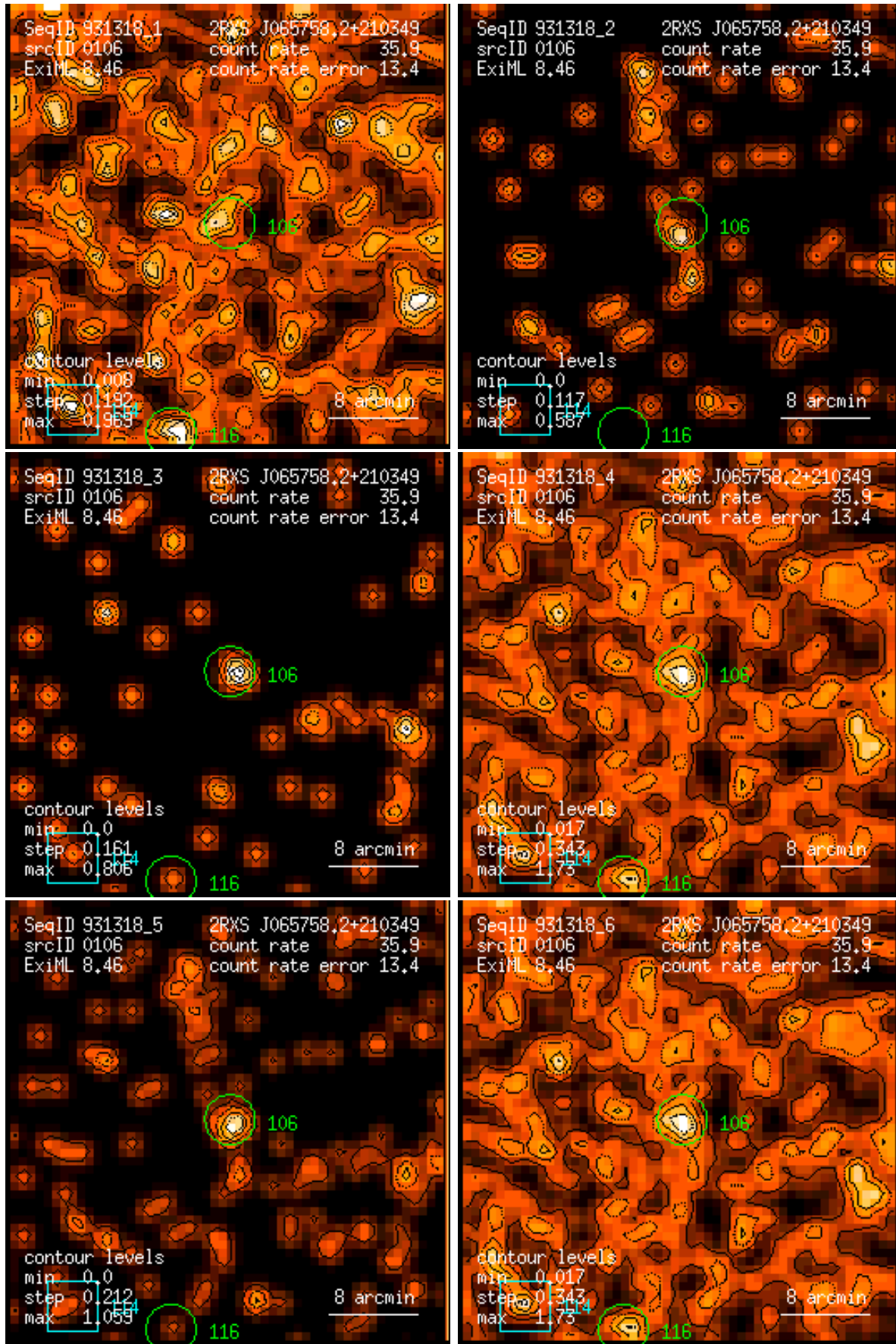
Figure 106: RASS 931318: detection 0106: band rate images, Gaussian filter: (1) PSPC channels 11 – 41, (2) 52 – 90, (3) 91 – 201, (4) 11 – 235, (5) 52 – 201, (6) 11 – 201. Broad band rates in counts/ks. Band rate contour levels in counts/ks/arcmin 2 .
