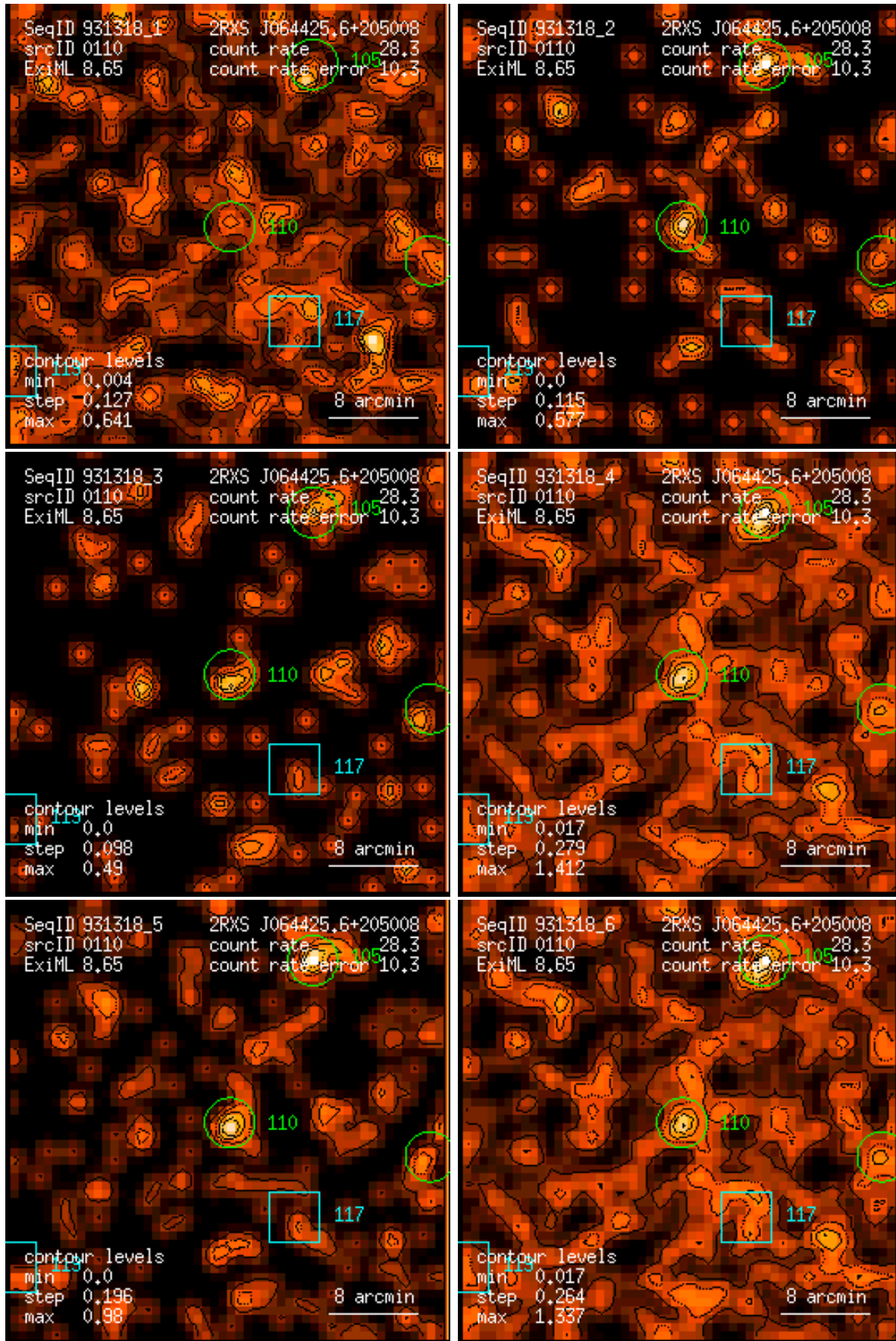
Figure 110: RASS 931318: detection 0110: band rate images, Gaussian filter: (1) PSPC channels 11 – 41, (2) 52 – 90, (3) 91 – 201, (4) 11 – 235, (5) 52 – 201, (6) 11 – 201. Broad band rates in counts/ks. Band rate contour levels in counts/ks/arcmin 2 .
