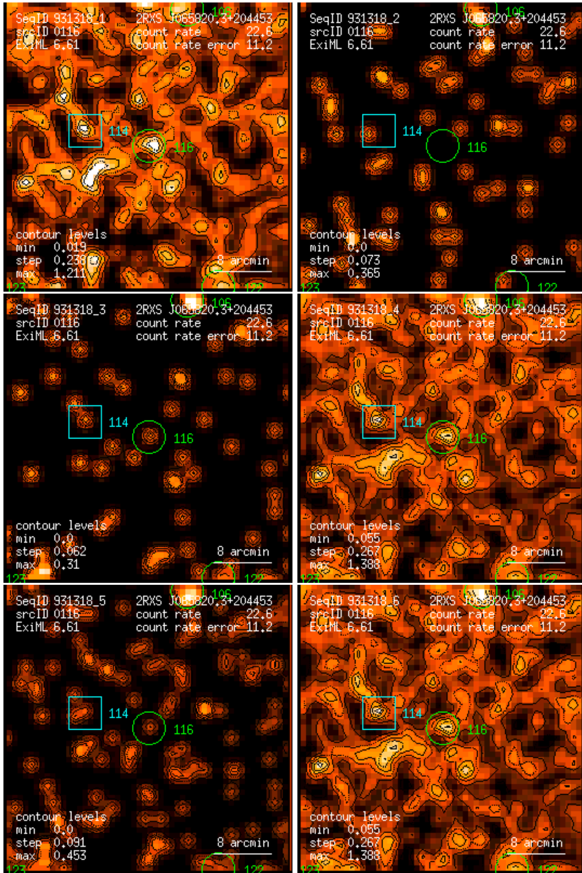
Figure 116: RASS 931318: detection 0116: band rate images, Gaussian filter: (1) PSPC channels 11 – 41, (2) 52 – 90, (3) 91 – 201, (4) 11 – 235, (5) 52 – 201, (6) 11 – 201. Broad band rates in counts/ks. Band rate contour levels in counts/ks/arcmin 2 .
