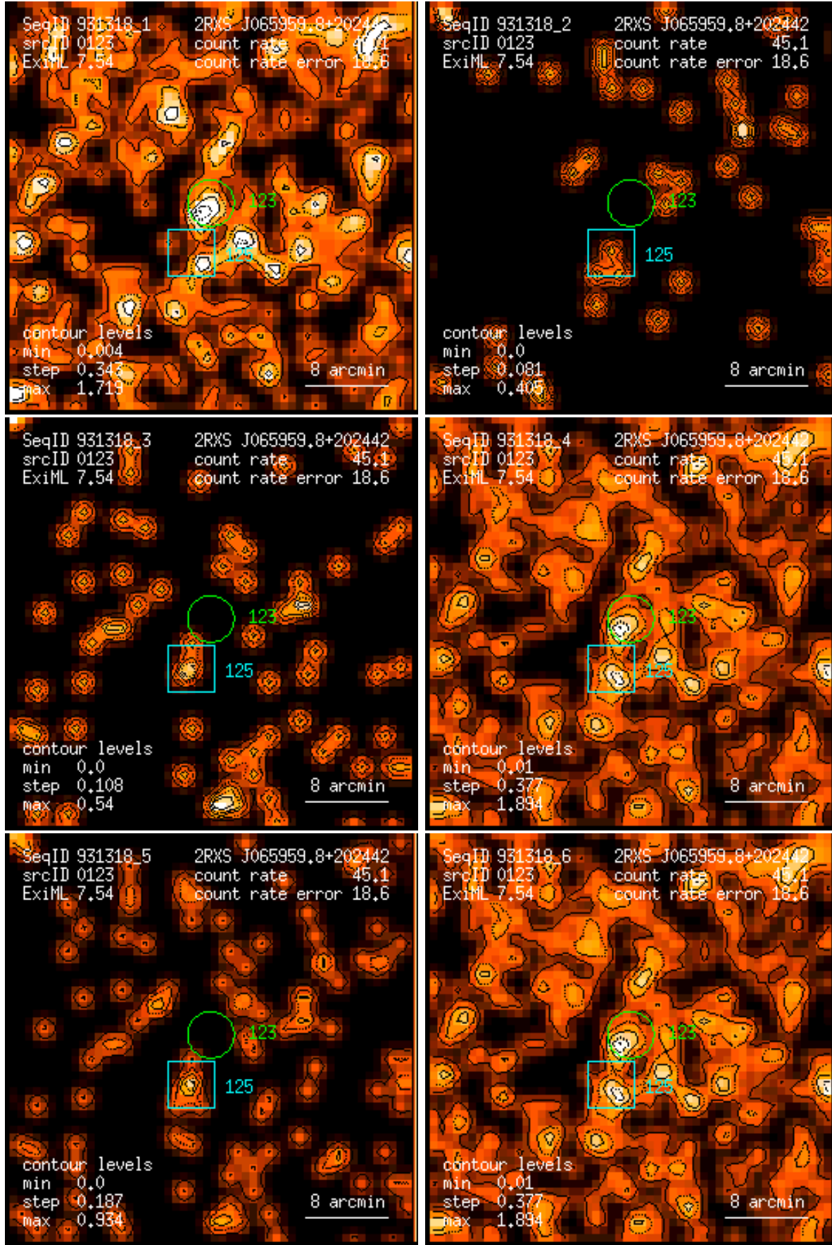
Figure 123: RASS 931318: detection 0123: band rate images, Gaussian filter: (1) PSPC channels 11 – 41, (2) 52 – 90, (3) 91 – 201, (4) 11 – 235, (5) 52 – 201, (6) 11 – 201. Broad band rates in counts/ks. Band rate contour levels in counts/ks/arcmin 2 .
