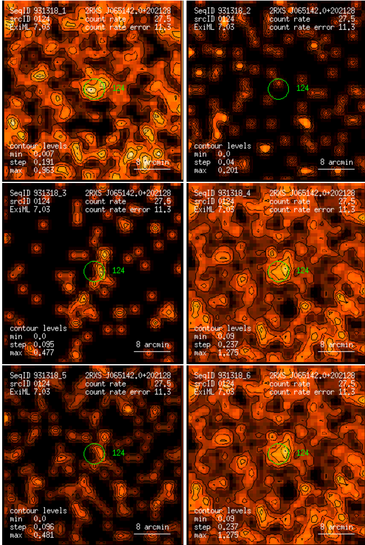
Figure 124: RASS 931318: detection 0124: band rate images, Gaussian filter: (1) PSPC channels 11 – 41, (2) 52 – 90, (3) 91 – 201, (4) 11 – 235, (5) 52 – 201, (6) 11 – 201. Broad band rates in counts/ks. Band rate contour levels in counts/ks/arcmin 2 .
