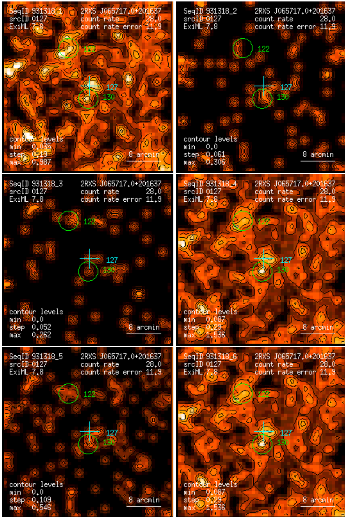
Figure 127: RASS 931318: detection 0127: band rate images, Gaussian filter: (1) PSPC channels 11 – 41, (2) 52 – 90, (3) 91 – 201, (4) 11 – 235, (5) 52 – 201, (6) 11 – 201. Broad band rates in counts/ks. Band rate contour levels in counts/ks/arcmin 2 .
