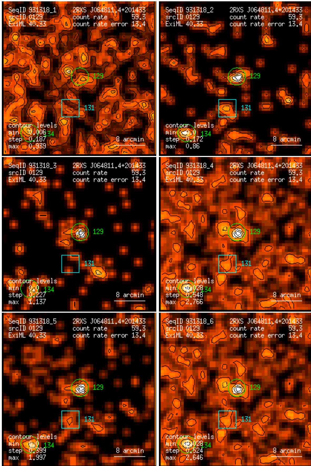
Figure 129: RASS 931318: detection 0129: band rate images, Gaussian filter: (1) PSPC channels 11 – 41, (2) 52 – 90, (3) 91 – 201, (4) 11 – 235, (5) 52 – 201, (6) 11 – 201. Broad band rates in counts/ks. Band rate contour levels in counts/ks/arcmin 2 .
