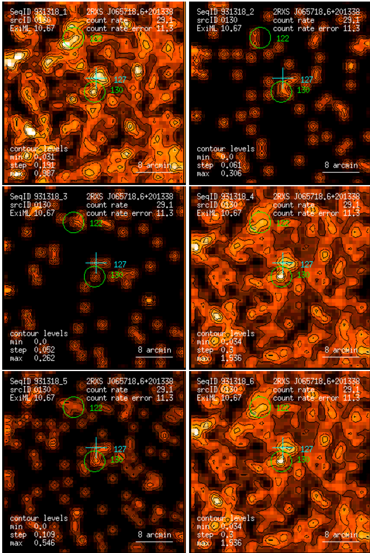
Figure 130: RASS 931318: detection 0130: band rate images, Gaussian filter: (1) PSPC channels 11 – 41, (2) 52 – 90, (3) 91 – 201, (4) 11 – 235, (5) 52 – 201, (6) 11 – 201. Broad band rates in counts/ks. Band rate contour levels in counts/ks/arcmin 2 .
