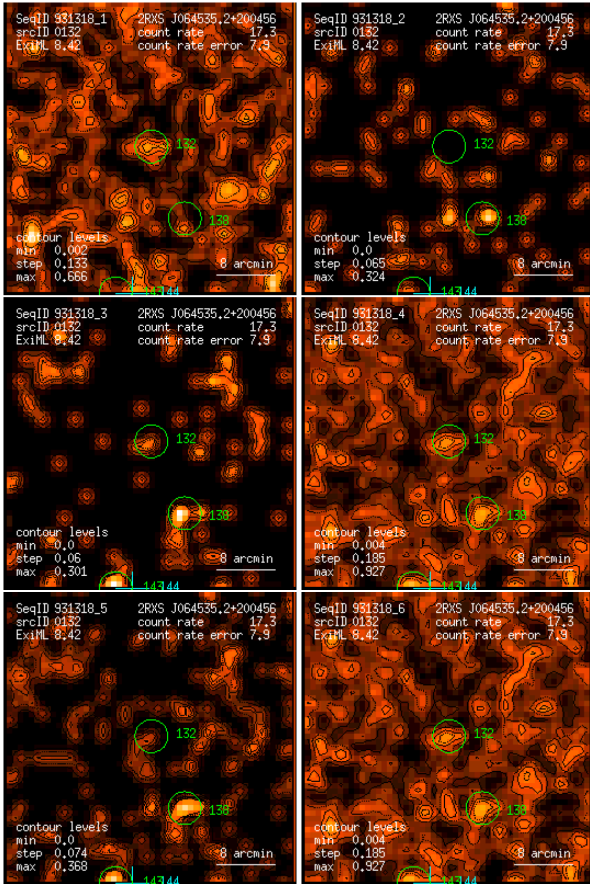
Figure 132: RASS 931318: detection 0132: band rate images, Gaussian filter: (1) PSPC channels 11 – 41, (2) 52 – 90, (3) 91 – 201, (4) 11 – 235, (5) 52 – 201, (6) 11 – 201. Broad band rates in counts/ks. Band rate contour levels in counts/ks/arcmin 2 .
