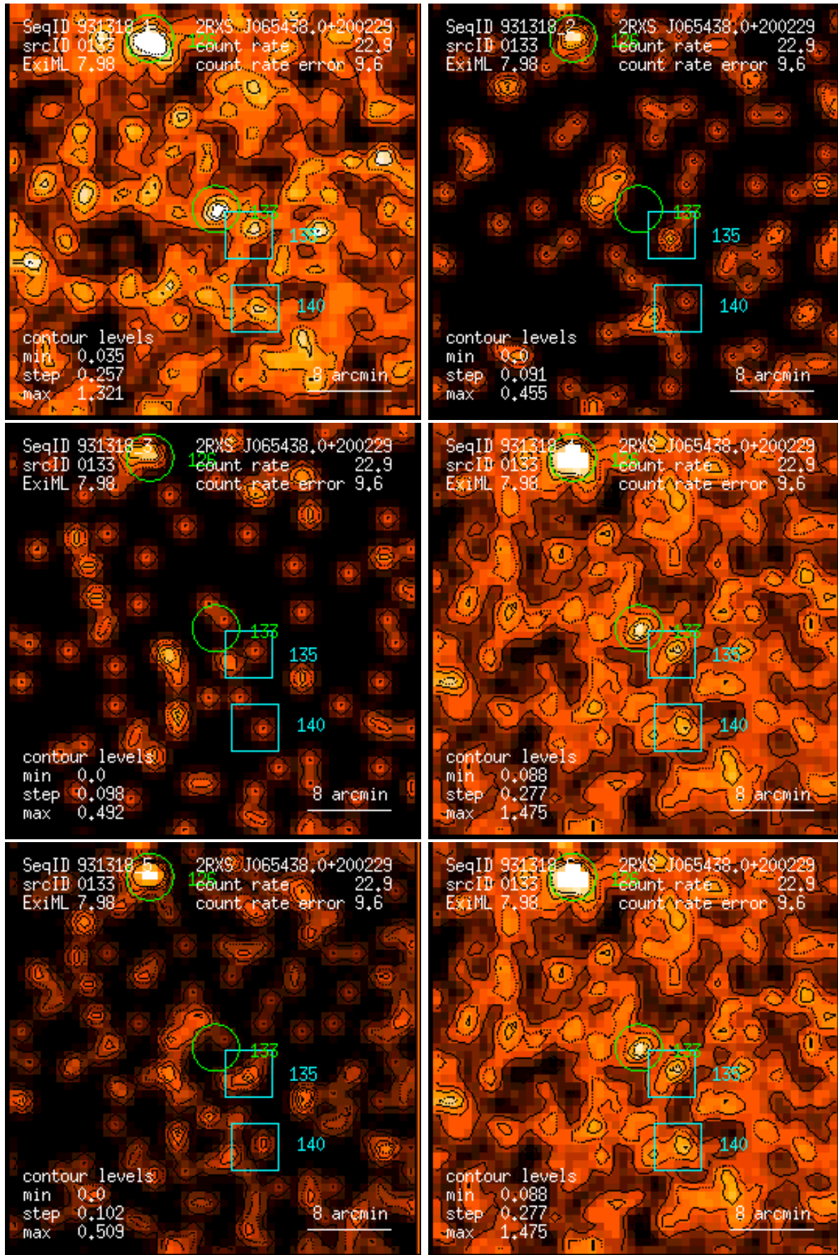
Figure 133: RASS 931318: detection 0133: band rate images, Gaussian filter: (1) PSPC channels 11 – 41, (2) 52 – 90, (3) 91 – 201, (4) 11 – 235, (5) 52 – 201, (6) 11 – 201. Broad band rates in counts/ks. Band rate contour levels in counts/ks/arcmin 2 .
