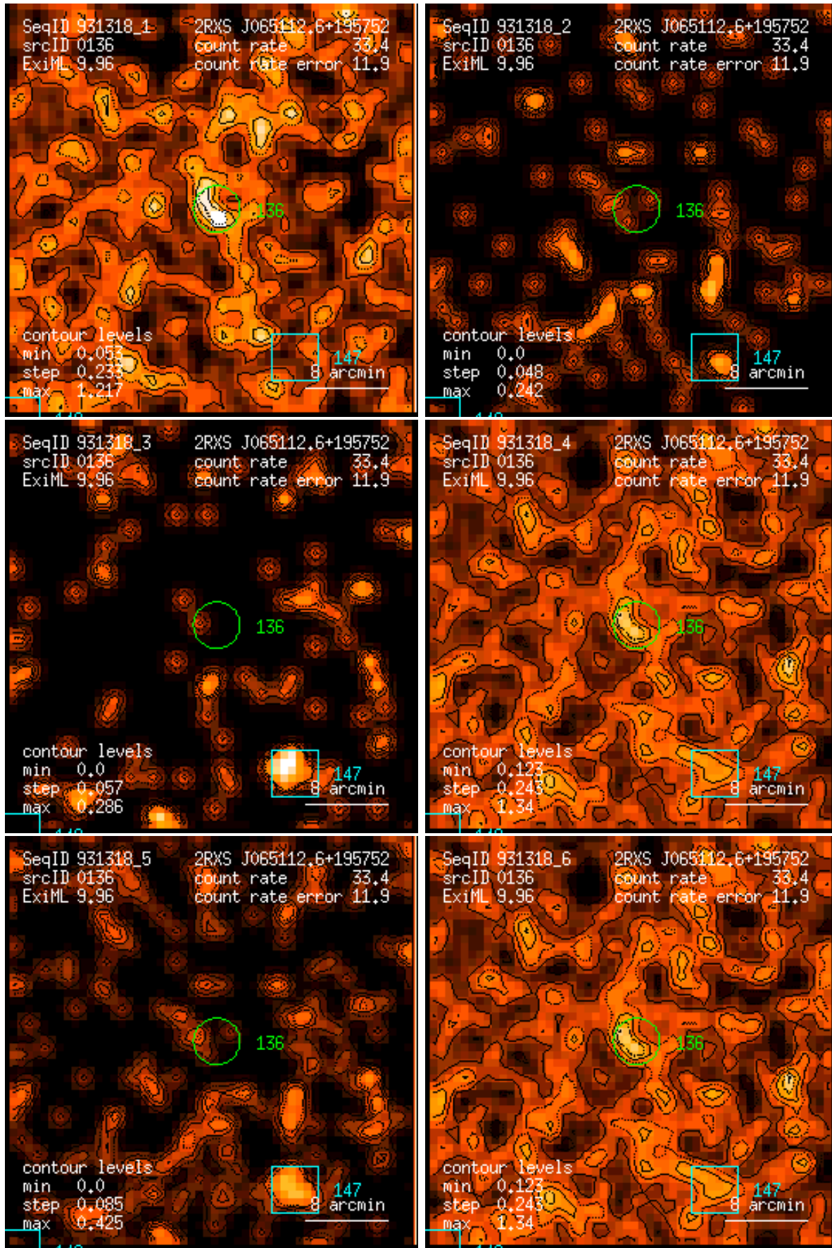
Figure 136: RASS 931318: detection 0136: band rate images, Gaussian filter: (1) PSPC channels 11 – 41, (2) 52 – 90, (3) 91 – 201, (4) 11 – 235, (5) 52 – 201, (6) 11 – 201. Broad band rates in counts/ks. Band rate contour levels in counts/ks/arcmin 2 .
