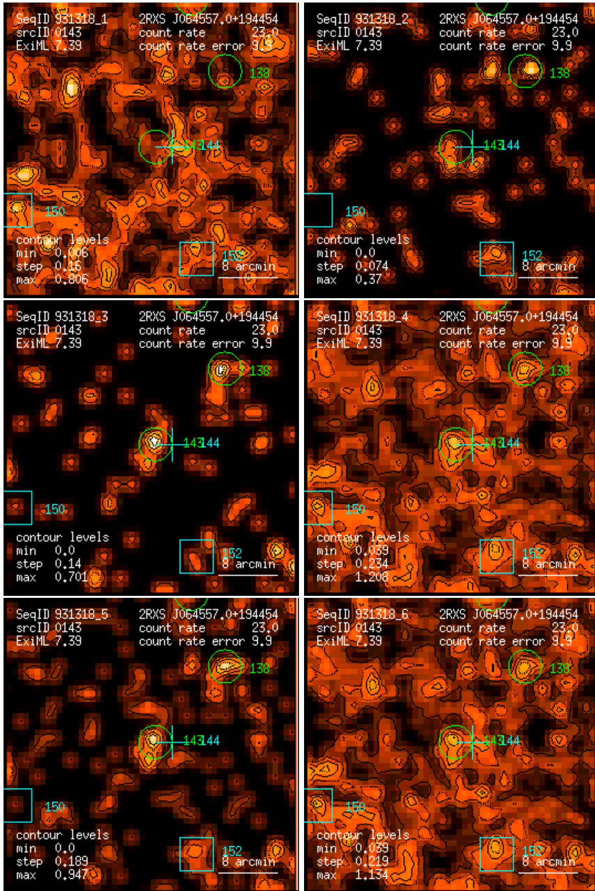
Figure 143: RASS 931318: detection 0143: band rate images, Gaussian filter: (1) PSPC channels 11 – 41, (2) 52 – 90, (3) 91 – 201, (4) 11 – 235, (5) 52 – 201, (6) 11 – 201. Broad band rates in counts/ks. Band rate contour levels in counts/ks/arcmin 2 .
