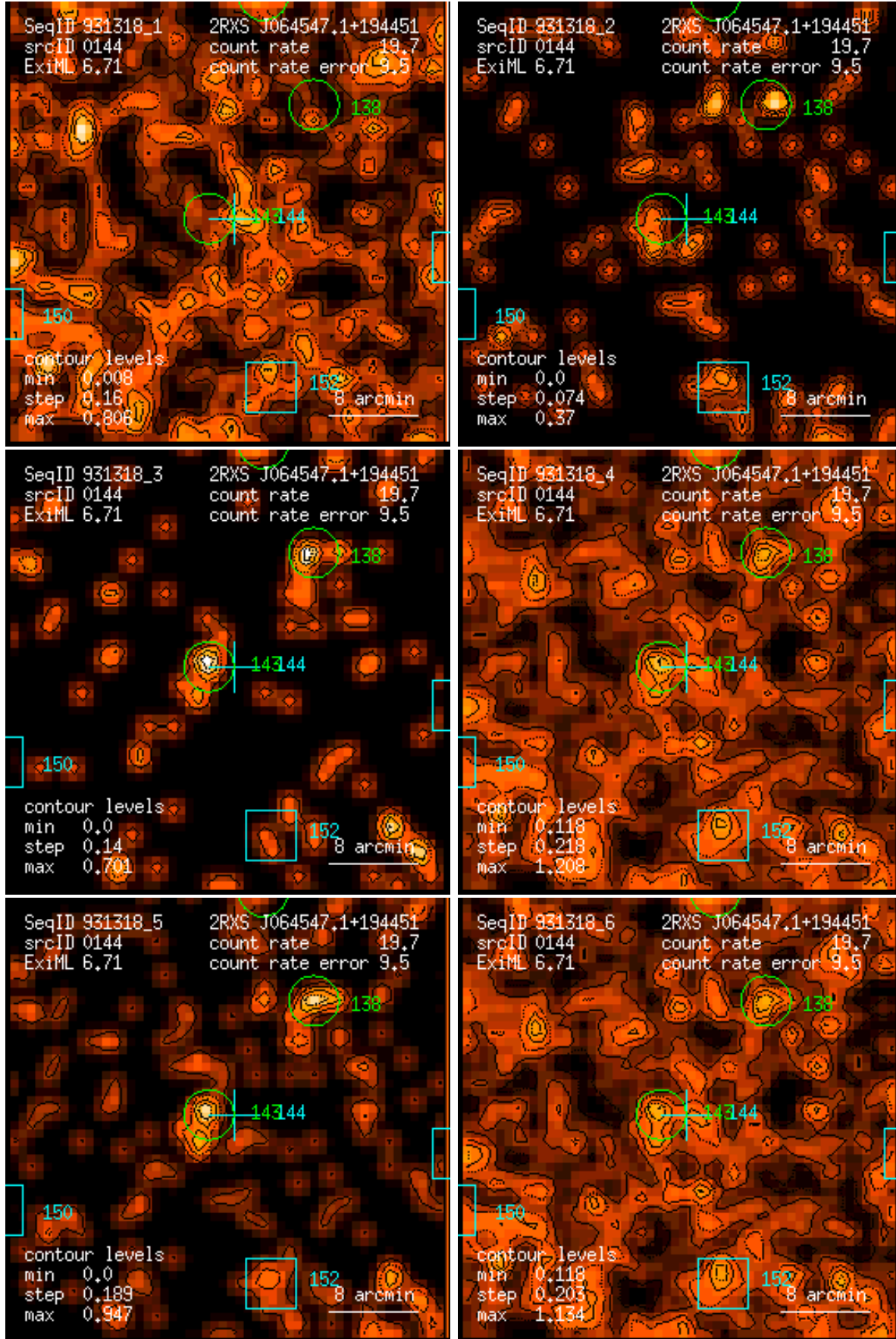
Figure 144: RASS 931318: detection 0144: band rate images, Gaussian filter: (1) PSPC channels 11 – 41, (2) 52 – 90, (3) 91 – 201, (4) 11 – 235, (5) 52 – 201, (6) 11 – 201. Broad band rates in counts/ks. Band rate contour levels in counts/ks/arcmin 2 .
