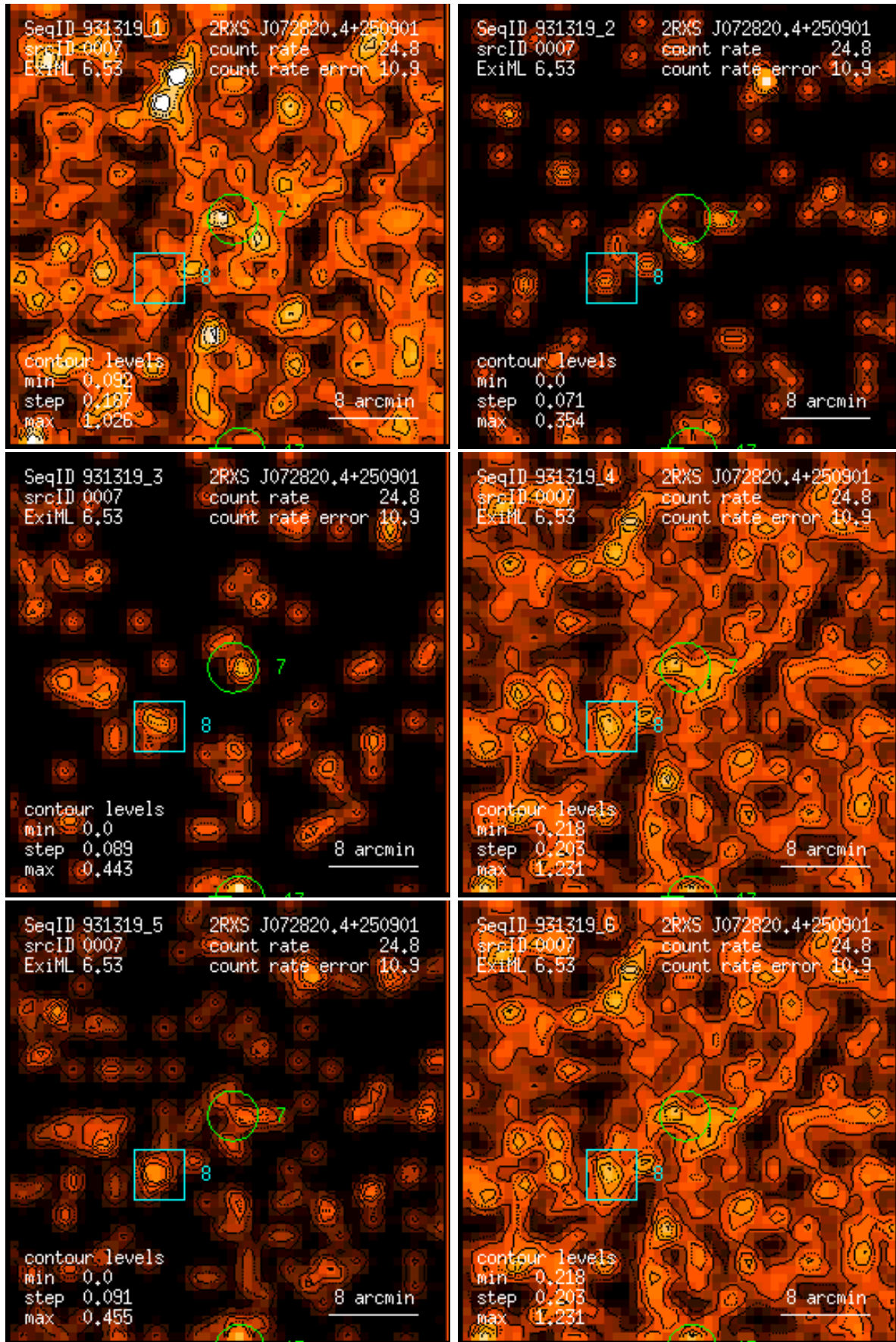
Figure 7: RASS 931319: detection 0007: band rate images, Gaussian filter: (1) PSPC channels 11 – 41, (2) 52 – 90, (3) 91 – 201, (4) 11 – 235, (5) 52 – 201, (6) 11 – 201. Broad band rates in counts/ks. Band rate contour levels in counts/ks/arcmin 2 .
