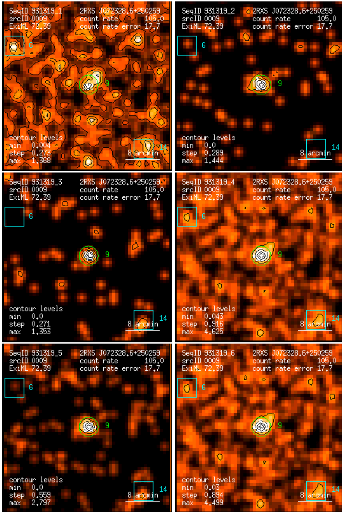
Figure 9: RASS 931319: detection 0009: band rate images, Gaussian filter: (1) PSPC channels 11 – 41, (2) 52 – 90, (3) 91 – 201, (4) 11 – 235, (5) 52 – 201, (6) 11 – 201. Broad band rates in counts/ks. Band rate contour levels in counts/ks/arcmin 2 .
