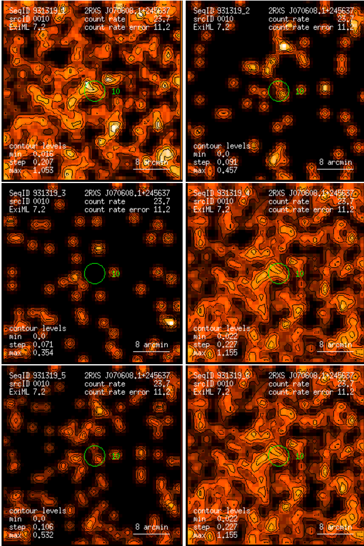
Figure 10: RASS 931319: detection 0010: band rate images, Gaussian filter: (1) PSPC channels 11 – 41, (2) 52 – 90, (3) 91 – 201, (4) 11 – 235, (5) 52 – 201, (6) 11 – 201. Broad band rates in counts/ks. Band rate contour levels in counts/ks/arcmin 2 .
