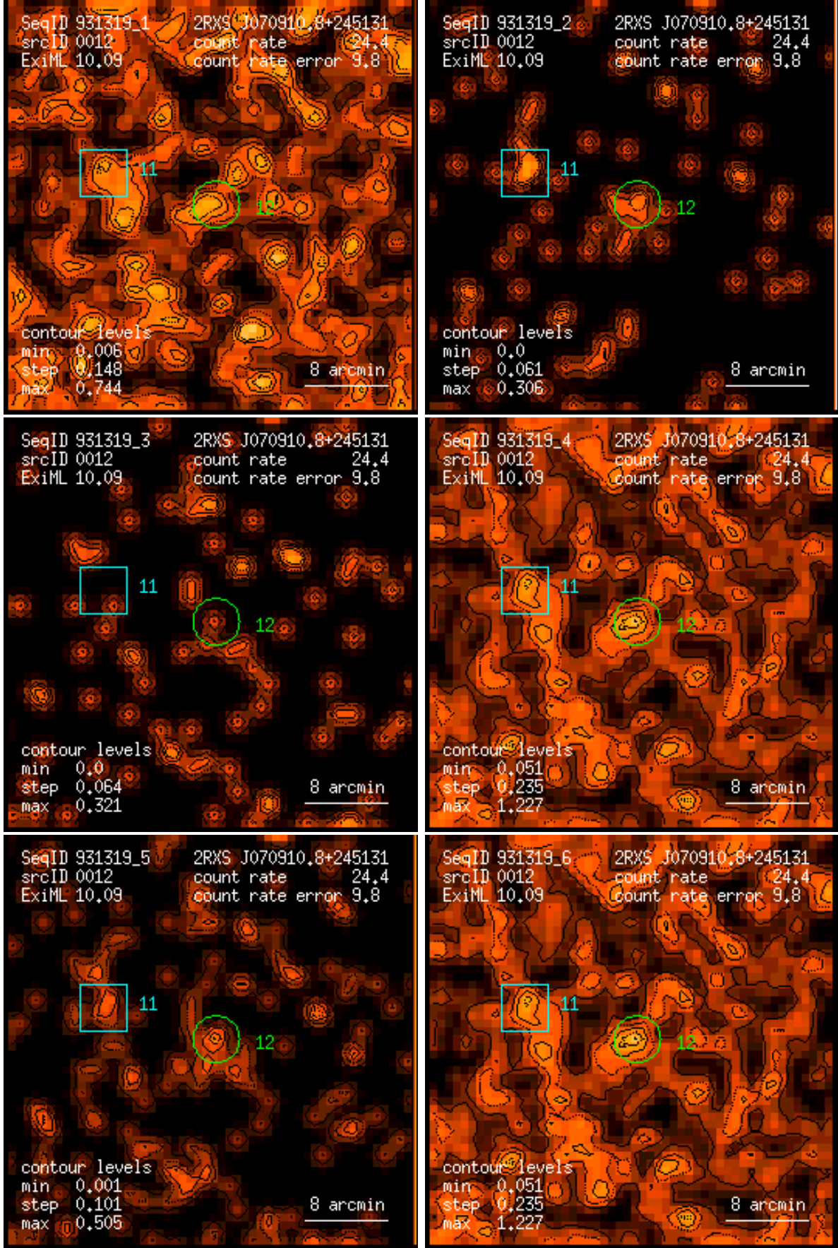
Figure 12: RASS 931319: detection 0012: band rate images, Gaussian filter: (1) PSPC channels 11 – 41, (2) 52 – 90, (3) 91 – 201, (4) 11 – 235, (5) 52 – 201, (6) 11 – 201. Broad band rates in counts/ks. Band rate contour levels in counts/ks/arcmin 2 .
