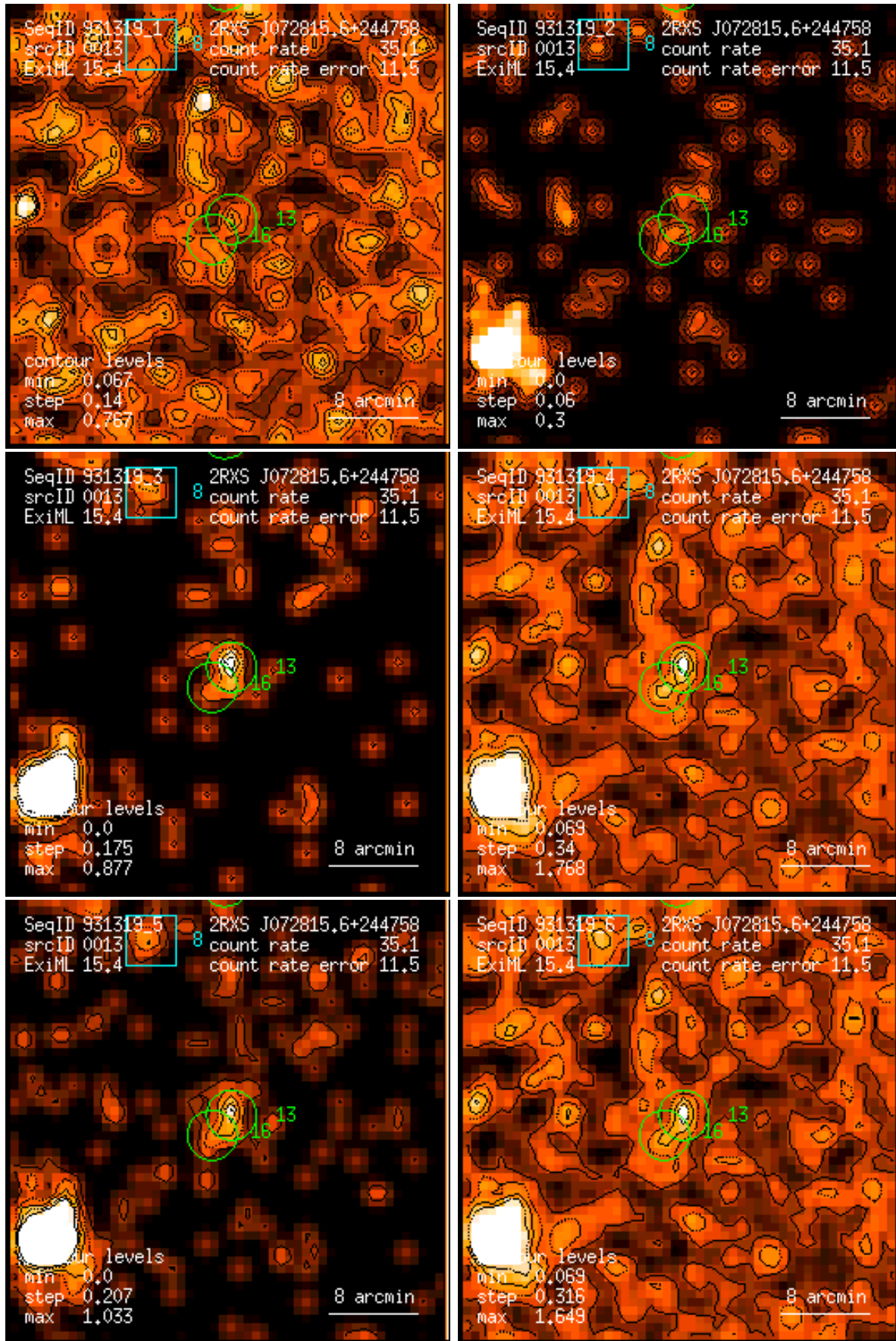
Figure 13: RASS 931319: detection 0013: band rate images, Gaussian filter: (1) PSPC channels 11 – 41, (2) 52 – 90, (3) 91 – 201, (4) 11 – 235, (5) 52 – 201, (6) 11 – 201. Broad band rates in counts/ks. Band rate contour levels in counts/ks/arcmin 2 .
