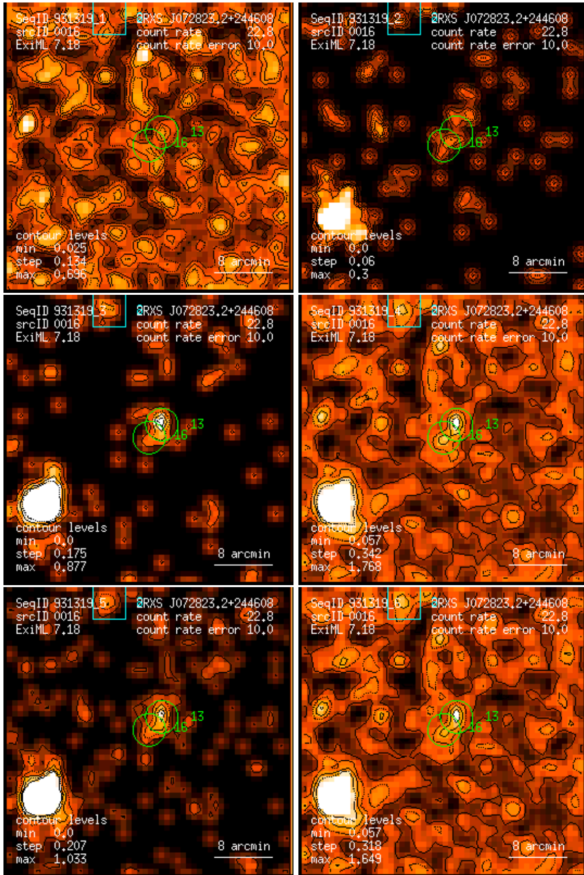
Figure 16: RASS 931319: detection 0016: band rate images, Gaussian filter: (1) PSPC channels 11 – 41, (2) 52 – 90, (3) 91 – 201, (4) 11 – 235, (5) 52 – 201, (6) 11 – 201. Broad band rates in counts/ks. Band rate contour levels in counts/ks/arcmin 2 .
