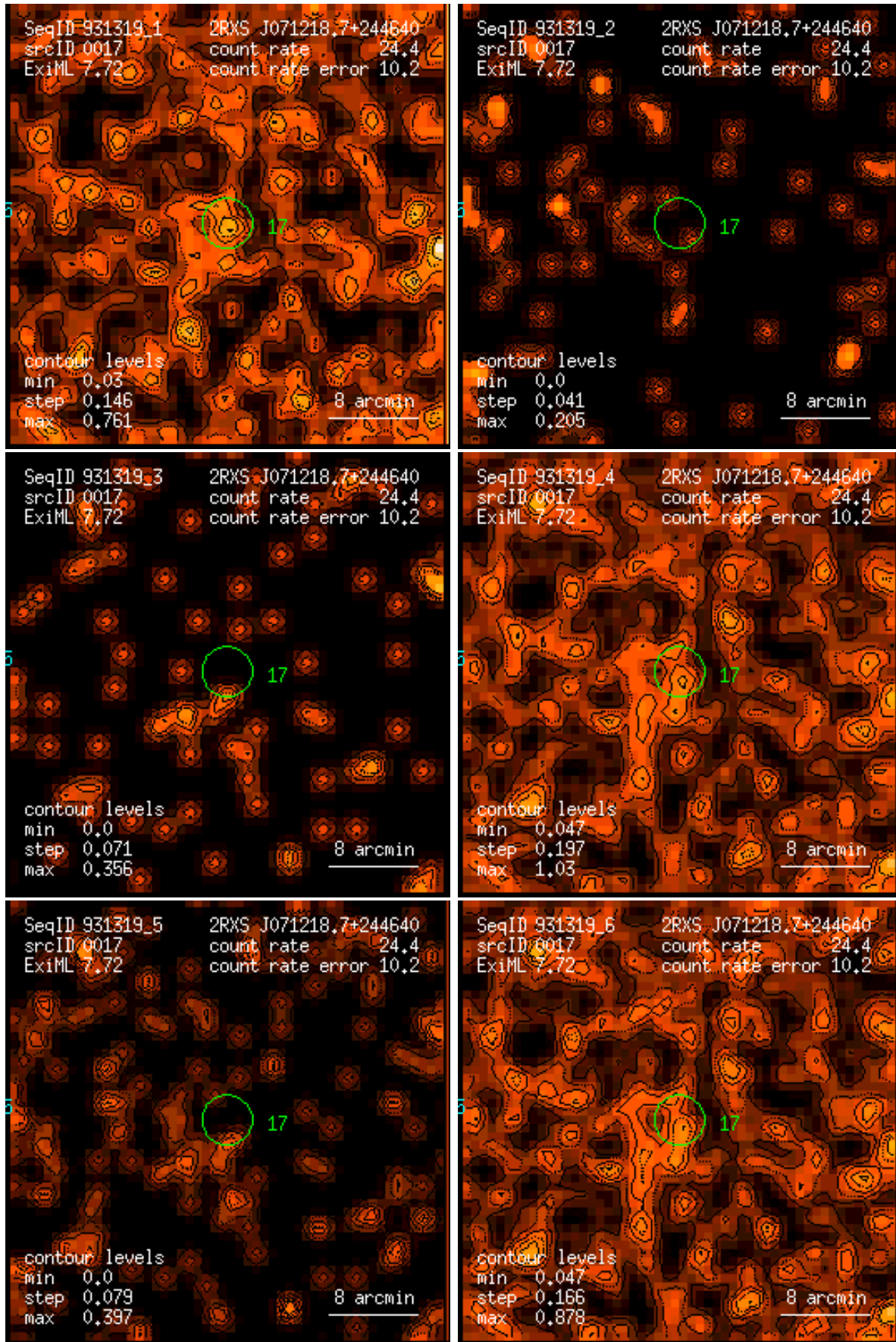
Figure 17: RASS 931319: detection 0017: band rate images, Gaussian filter: (1) PSPC channels 11 – 41, (2) 52 – 90, (3) 91 – 201, (4) 11 – 235, (5) 52 – 201, (6) 11 – 201. Broad band rates in counts/ks. Band rate contour levels in counts/ks/arcmin 2 .
