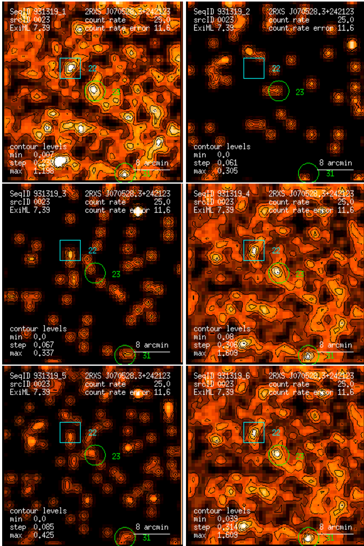
Figure 23: RASS 931319: detection 0023: band rate images, Gaussian filter: (1) PSPC channels 11 – 41, (2) 52 – 90, (3) 91 – 201, (4) 11 – 235, (5) 52 – 201, (6) 11 – 201. Broad band rates in counts/ks. Band rate contour levels in counts/ks/arcmin 2 .
