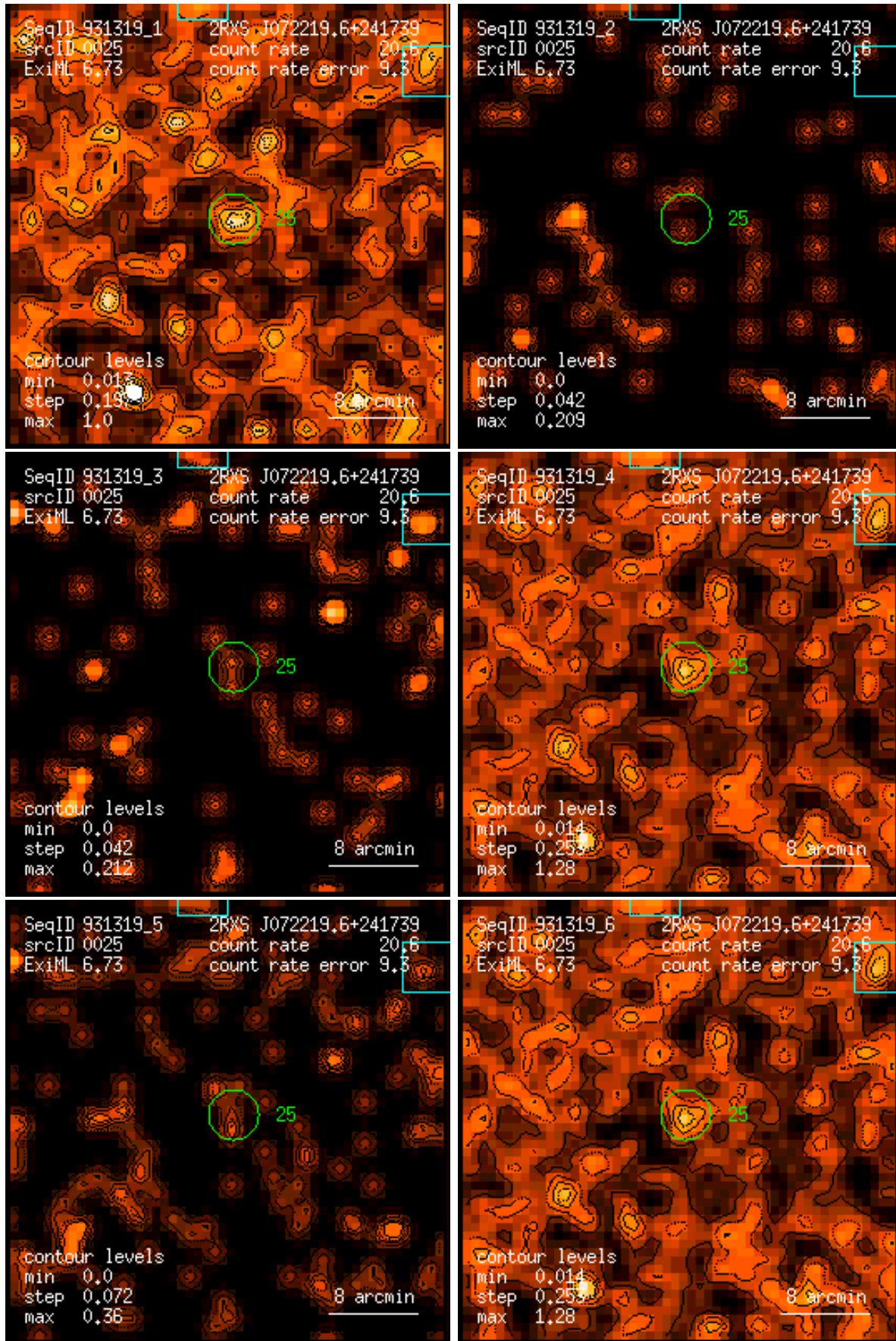
Figure 25: RASS 931319: detection 0025: band rate images, Gaussian filter: (1) PSPC channels 11 – 41, (2) 52 – 90, (3) 91 – 201, (4) 11 – 235, (5) 52 – 201, (6) 11 – 201. Broad band rates in counts/ks. Band rate contour levels in counts/ks/arcmin 2 .
