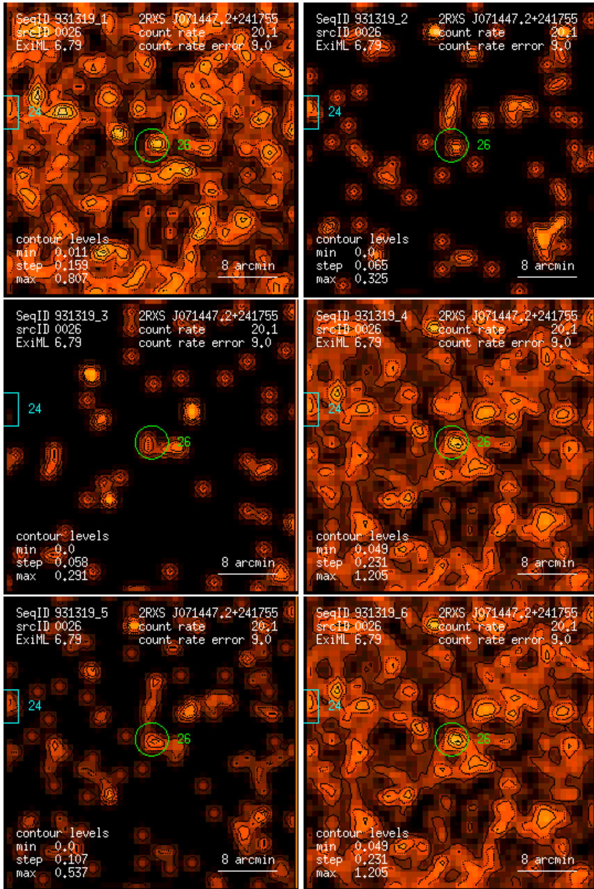
Figure 26: RASS 931319: detection 0026: band rate images, Gaussian filter: (1) PSPC channels 11 – 41, (2) 52 – 90, (3) 91 – 201, (4) 11 – 235, (5) 52 – 201, (6) 11 – 201. Broad band rates in counts/ks. Band rate contour levels in counts/ks/arcmin 2 .
