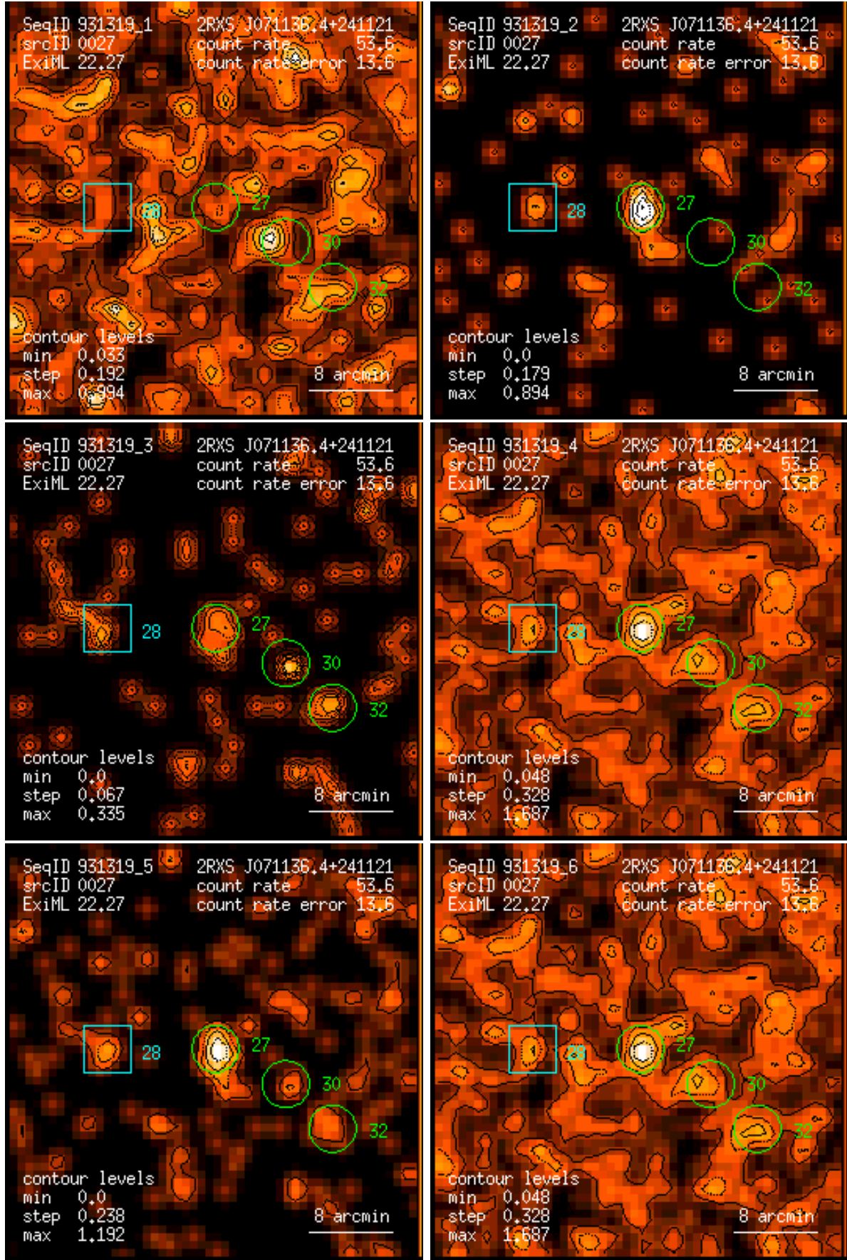
Figure 27: RASS 931319: detection 0027: band rate images, Gaussian filter: (1) PSPC channels 11 – 41, (2) 52 – 90, (3) 91 – 201, (4) 11 – 235, (5) 52 – 201, (6) 11 – 201. Broad band rates in counts/ks. Band rate contour levels in counts/ks/arcmin 2 .
