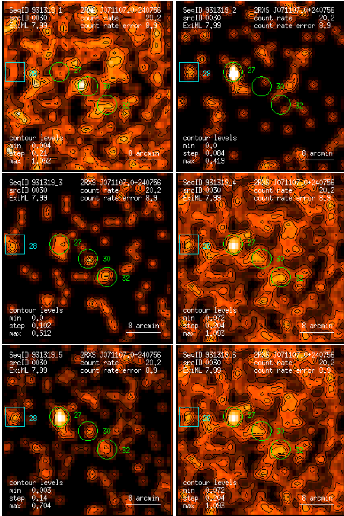
Figure 30: RASS 931319: detection 0030: band rate images, Gaussian filter: (1) PSPC channels 11 – 41, (2) 52 – 90, (3) 91 – 201, (4) 11 – 235, (5) 52 – 201, (6) 11 – 201. Broad band rates in counts/ks. Band rate contour levels in counts/ks/arcmin 2 .
