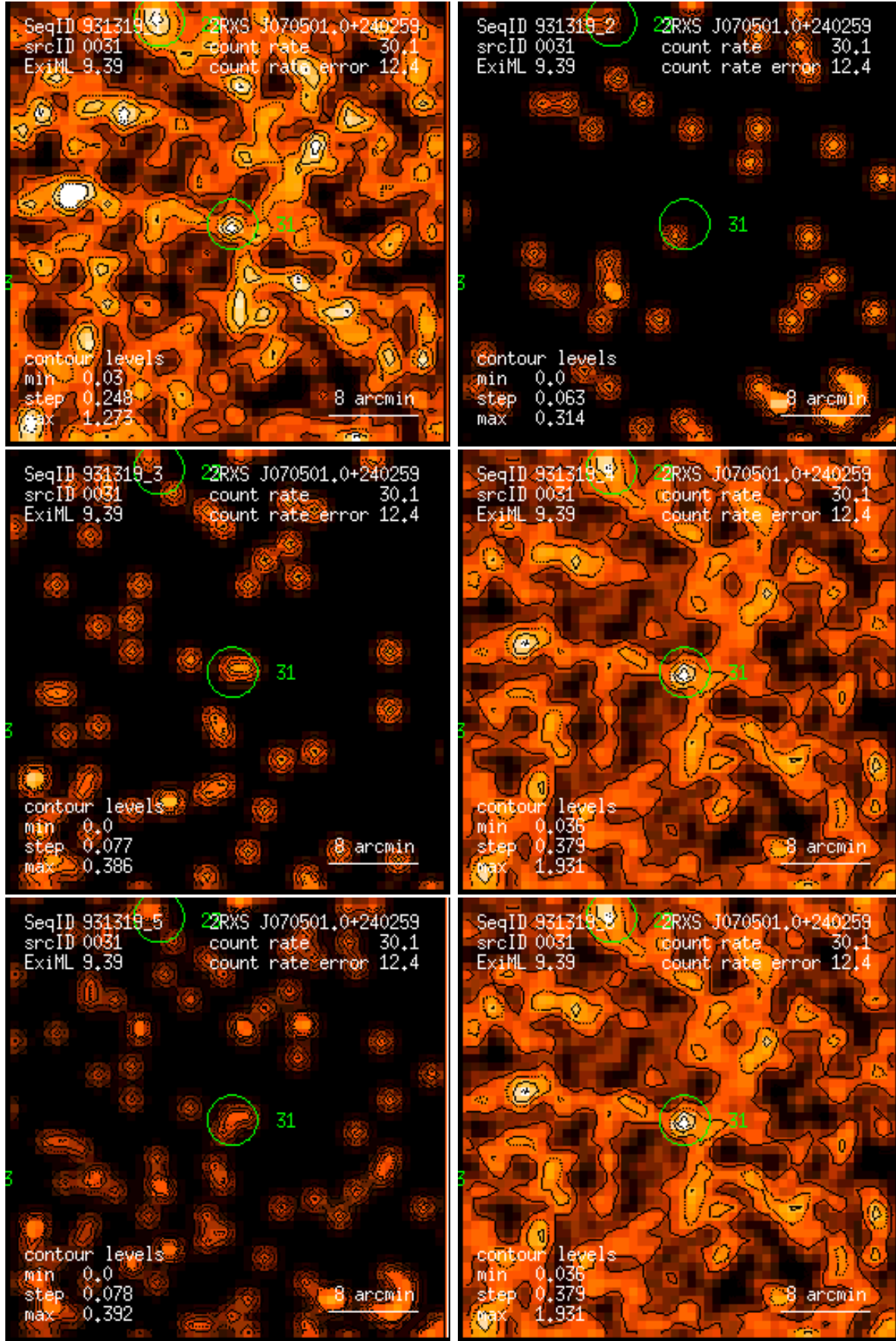
Figure 31: RASS 931319: detection 0031: band rate images, Gaussian filter: (1) PSPC channels 11 – 41, (2) 52 – 90, (3) 91 – 201, (4) 11 – 235, (5) 52 – 201, (6) 11 – 201. Broad band rates in counts/ks. Band rate contour levels in counts/ks/arcmin 2 .
