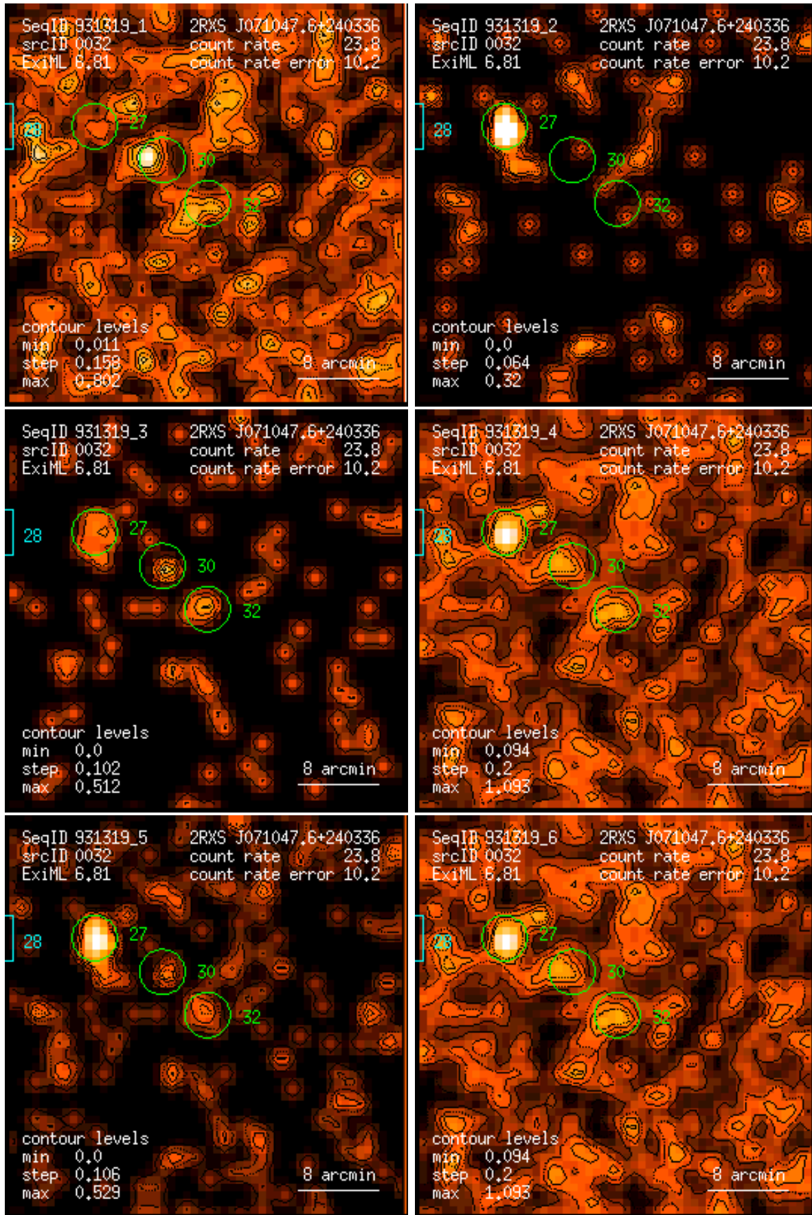
Figure 32: RASS 931319: detection 0032: band rate images, Gaussian filter: (1) PSPC channels 11 – 41, (2) 52 – 90, (3) 91 – 201, (4) 11 – 235, (5) 52 – 201, (6) 11 – 201. Broad band rates in counts/ks. Band rate contour levels in counts/ks/arcmin 2 .
