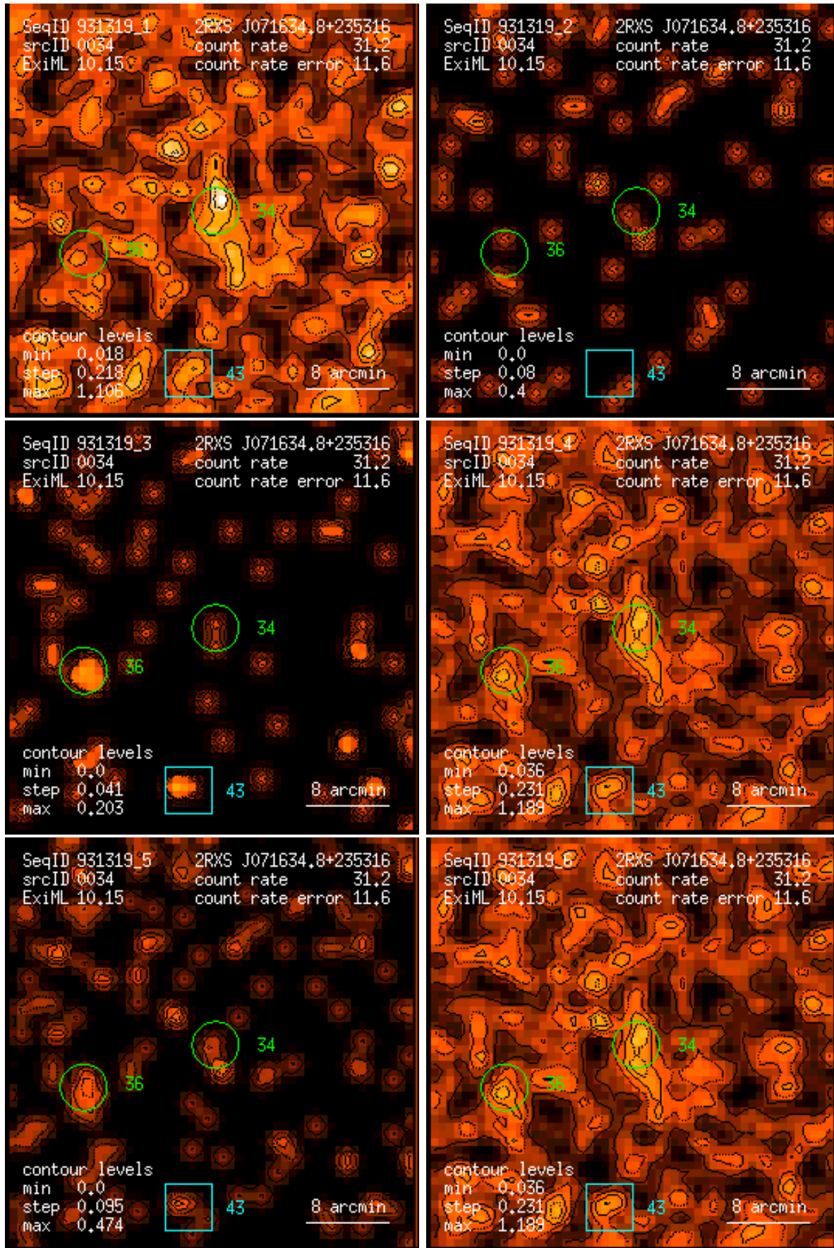
Figure 34: RASS 931319: detection 0034: band rate images, Gaussian filter: (1) PSPC channels 11 – 41, (2) 52 – 90, (3) 91 – 201, (4) 11 – 235, (5) 52 – 201, (6) 11 – 201. Broad band rates in counts/ks. Band rate contour levels in counts/ks/arcmin 2 .
