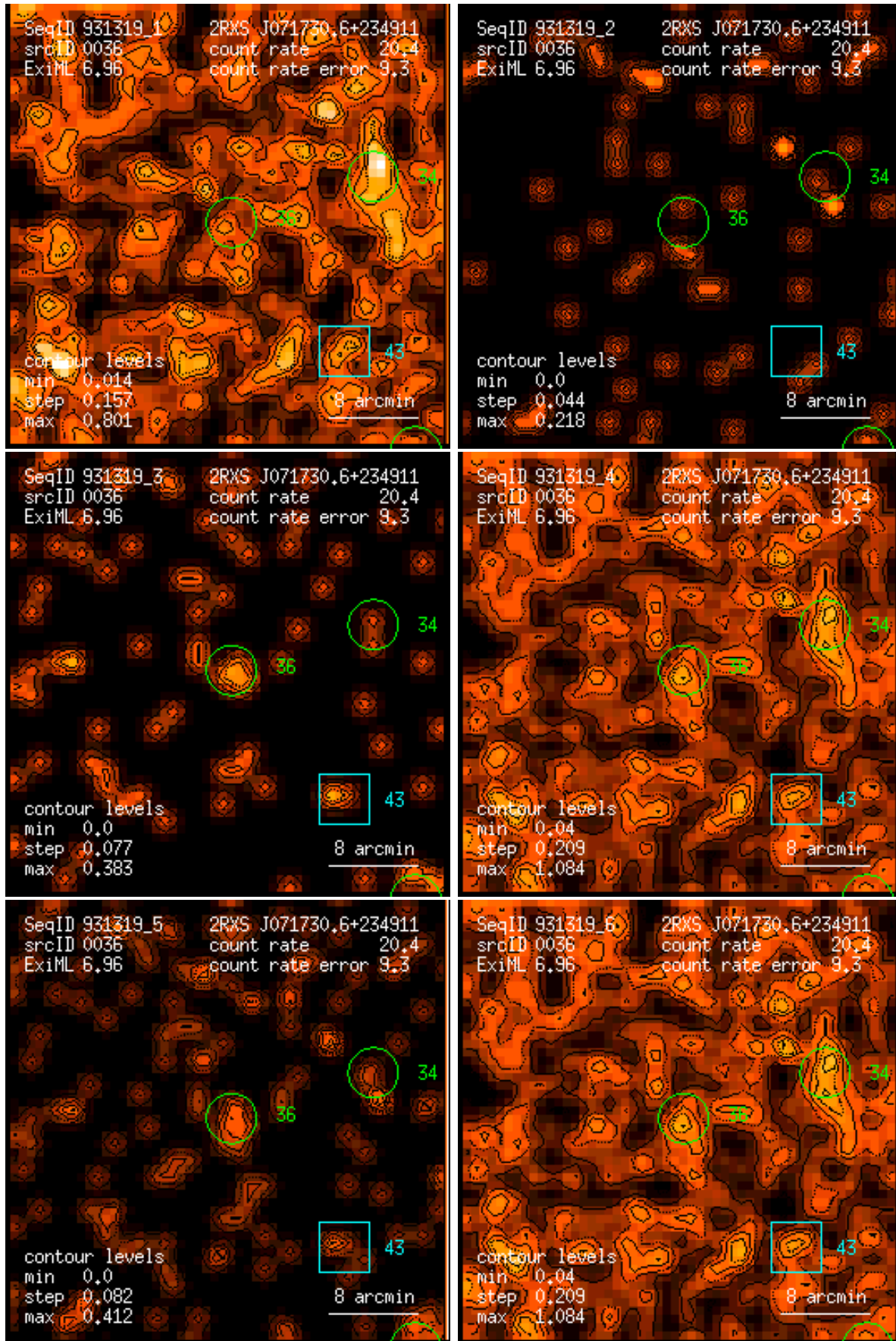
Figure 36: RASS 931319: detection 0036: band rate images, Gaussian filter: (1) PSPC channels 11 – 41, (2) 52 – 90, (3) 91 – 201, (4) 11 – 235, (5) 52 – 201, (6) 11 – 201. Broad band rates in counts/ks. Band rate contour levels in counts/ks/arcmin 2 .
