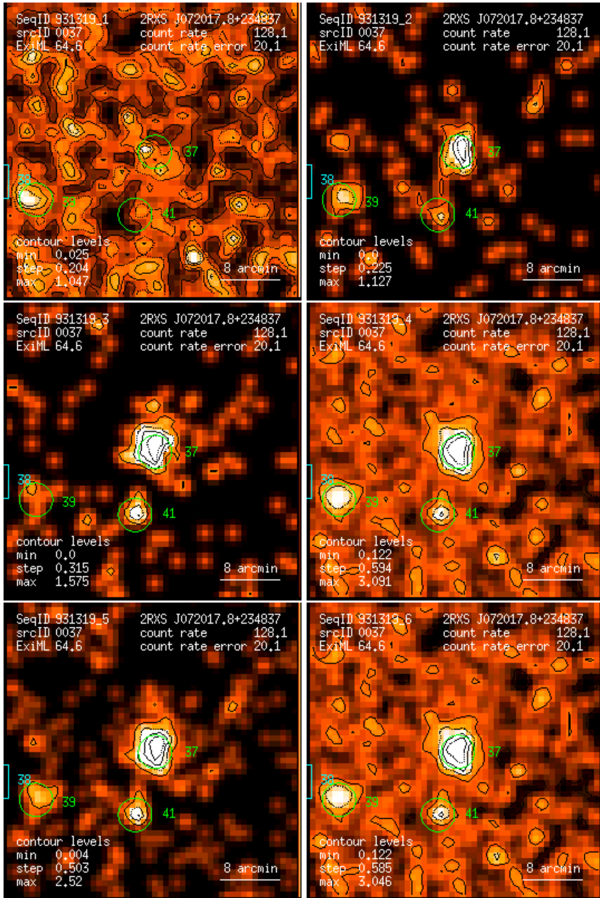
Figure 37: RASS 931319: detection 0037: band rate images, Gaussian filter: (1) PSPC channels 11 – 41, (2) 52 – 90, (3) 91 – 201, (4) 11 – 235, (5) 52 – 201, (6) 11 – 201. Broad band rates in counts/ks. Band rate contour levels in counts/ks/arcmin 2 .
