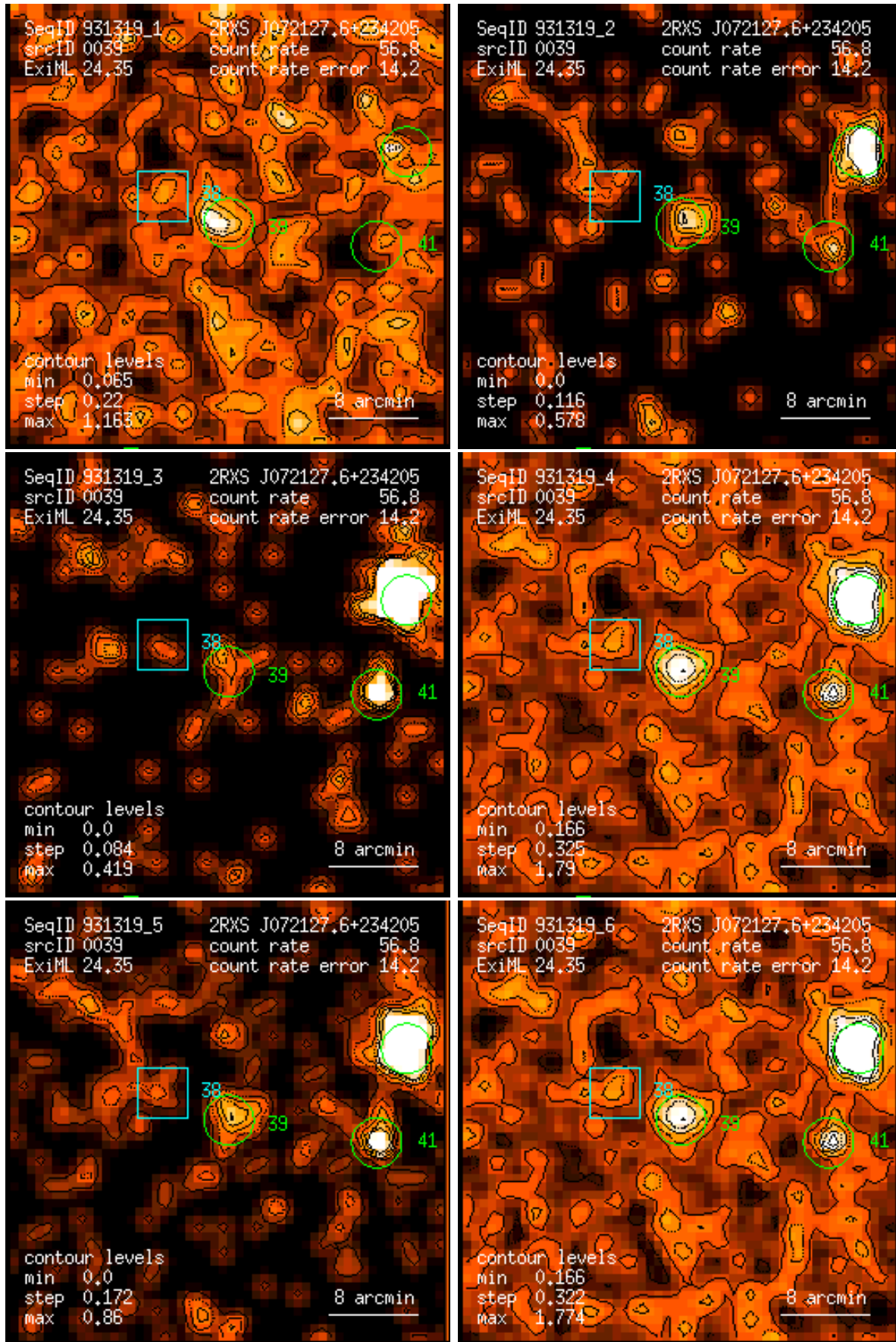
Figure 39: RASS 931319: detection 0039: band rate images, Gaussian filter: (1) PSPC channels 11 – 41, (2) 52 – 90, (3) 91 – 201, (4) 11 – 235, (5) 52 – 201, (6) 11 – 201. Broad band rates in counts/ks. Band rate contour levels in counts/ks/arcmin 2 .
